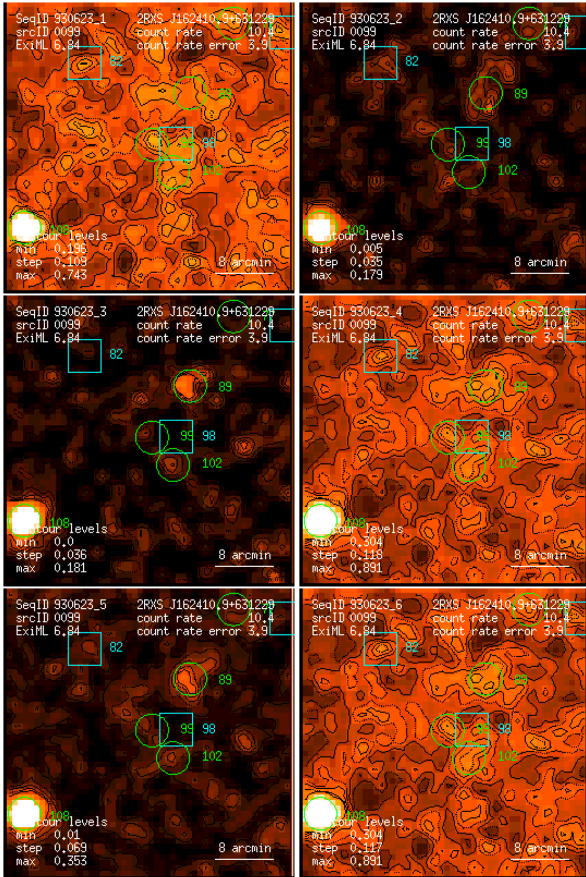
Figure 99: RASS 930623: detection 0099: band rate images, Gaussian filter: (1) PSPC channels 11 – 41, (2) 52 – 90, (3) 91 – 201, (4) 11 – 235, (5) 52 – 201, (6) 11 – 201. Broad band rates in counts/ks. Band rate contour levels in counts/ks/arcmin 2 .
