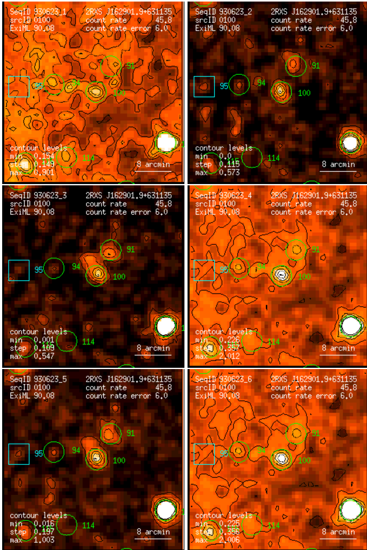
Figure 100: RASS 930623: detection 0100: band rate images, Gaussian filter: (1) PSPC channels 11 – 41, (2) 52 – 90, (3) 91 – 201, (4) 11 – 235, (5) 52 – 201, (6) 11 – 201. Broad band rates in counts/ks. Band rate contour levels in counts/ks/arcmin 2 .
