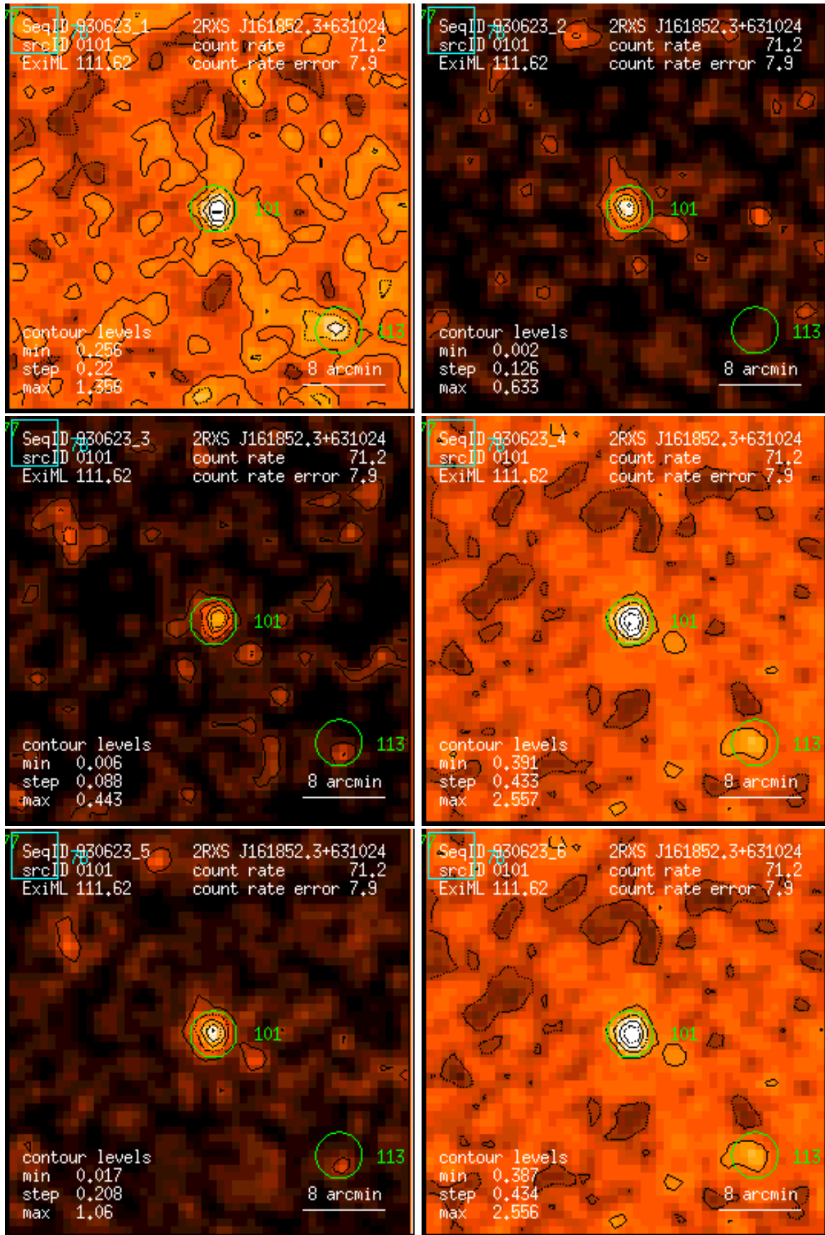
Figure 101: RASS 930623: detection 0101: band rate images, Gaussian filter: (1) PSPC channels 11 – 41, (2) 52 – 90, (3) 91 – 201, (4) 11 – 235, (5) 52 – 201, (6) 11 – 201. Broad band rates in counts/ks. Band rate contour levels in counts/ks/arcmin 2 .
