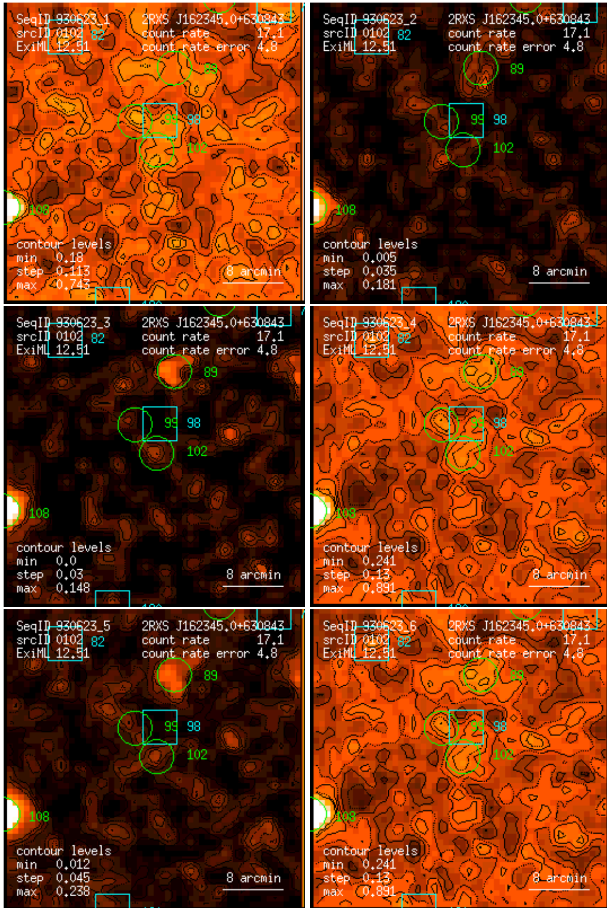
Figure 102: RASS 930623: detection 0102: band rate images, Gaussian filter: (1) PSPC channels 11 – 41, (2) 52 – 90, (3) 91 – 201, (4) 11 – 235, (5) 52 – 201, (6) 11 – 201. Broad band rates in counts/ks. Band rate contour levels in counts/ks/arcmin 2 .
