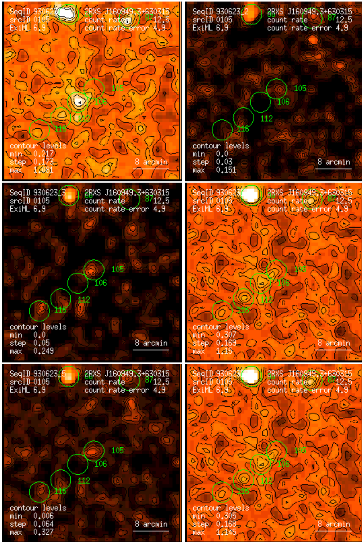
Figure 105: RASS 930623: detection 0105: band rate images, Gaussian filter: (1) PSPC channels 11 – 41, (2) 52 – 90, (3) 91 – 201, (4) 11 – 235, (5) 52 – 201, (6) 11 – 201. Broad band rates in counts/ks. Band rate contour levels in counts/ks/arcmin 2 .
