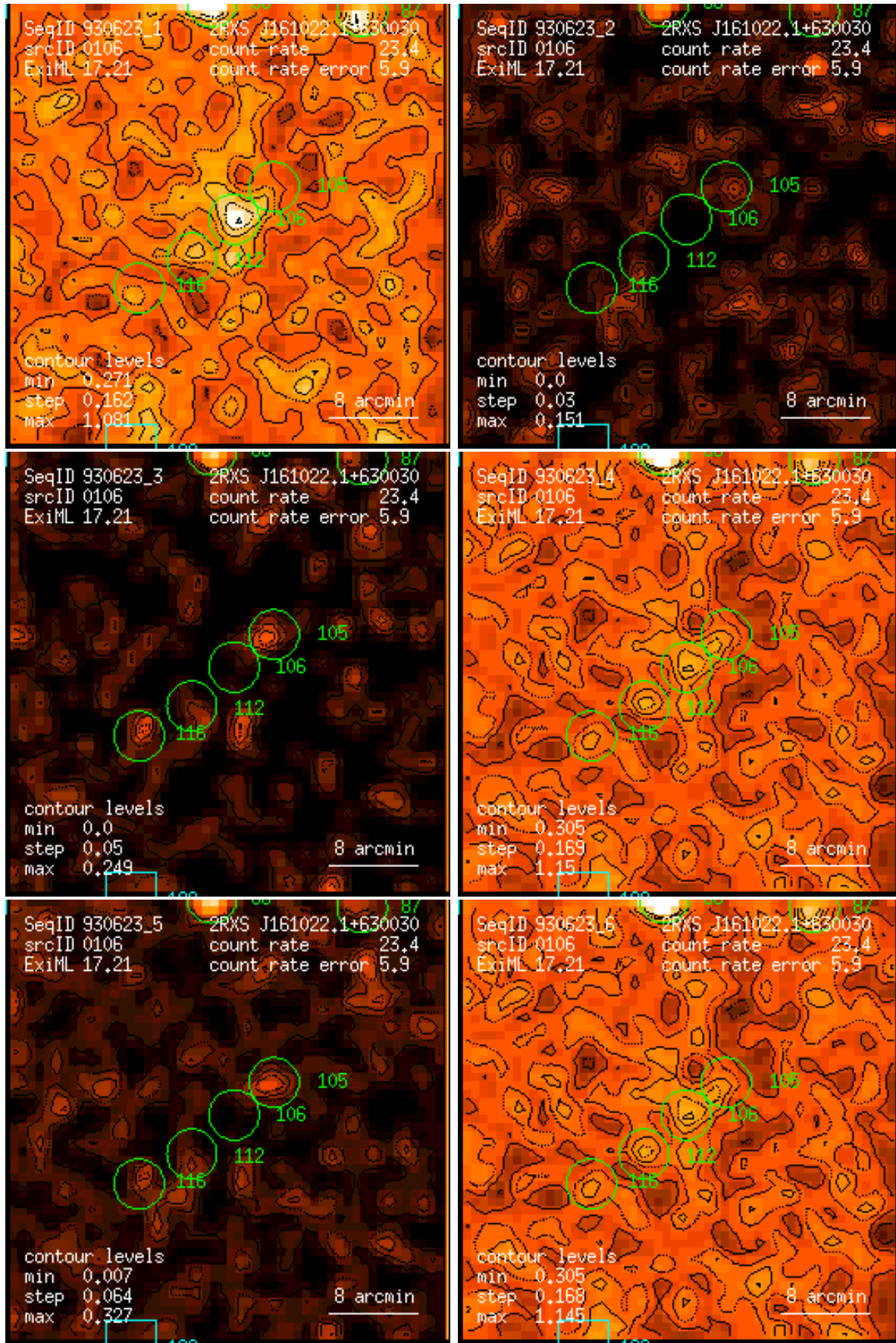
Figure 106: RASS 930623: detection 0106: band rate images, Gaussian filter: (1) PSPC channels 11 – 41, (2) 52 – 90, (3) 91 – 201, (4) 11 – 235, (5) 52 – 201, (6) 11 – 201. Broad band rates in counts/ks. Band rate contour levels in counts/ks/arcmin 2 .
