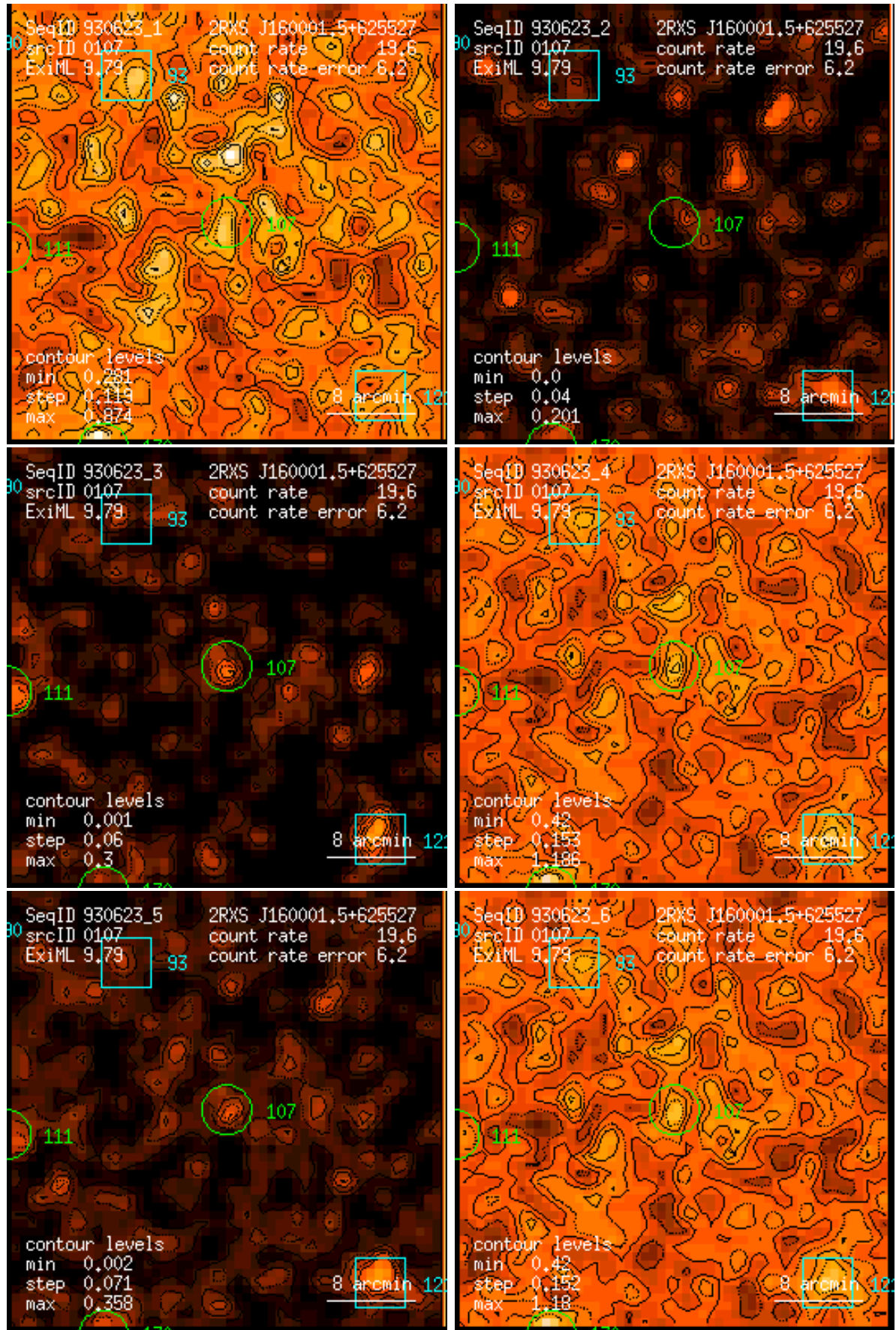
Figure 107: RASS 930623: detection 0107: band rate images, Gaussian filter: (1) PSPC channels 11 – 41, (2) 52 – 90, (3) 91 – 201, (4) 11 – 235, (5) 52 – 201, (6) 11 – 201. Broad band rates in counts/ks. Band rate contour levels in counts/ks/arcmin 2 .
