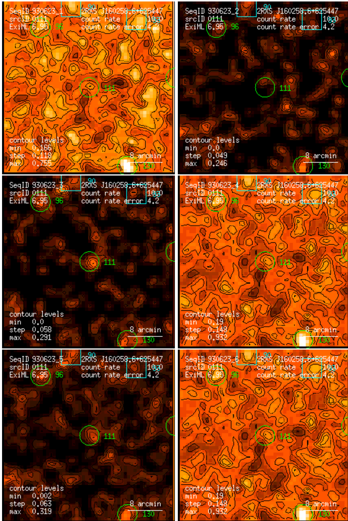
Figure 111: RASS 930623: detection 0111: band rate images, Gaussian filter: (1) PSPC channels 11 – 41, (2) 52 – 90, (3) 91 – 201, (4) 11 – 235, (5) 52 – 201, (6) 11 – 201. Broad band rates in counts/ks. Band rate contour levels in counts/ks/arcmin 2 .
