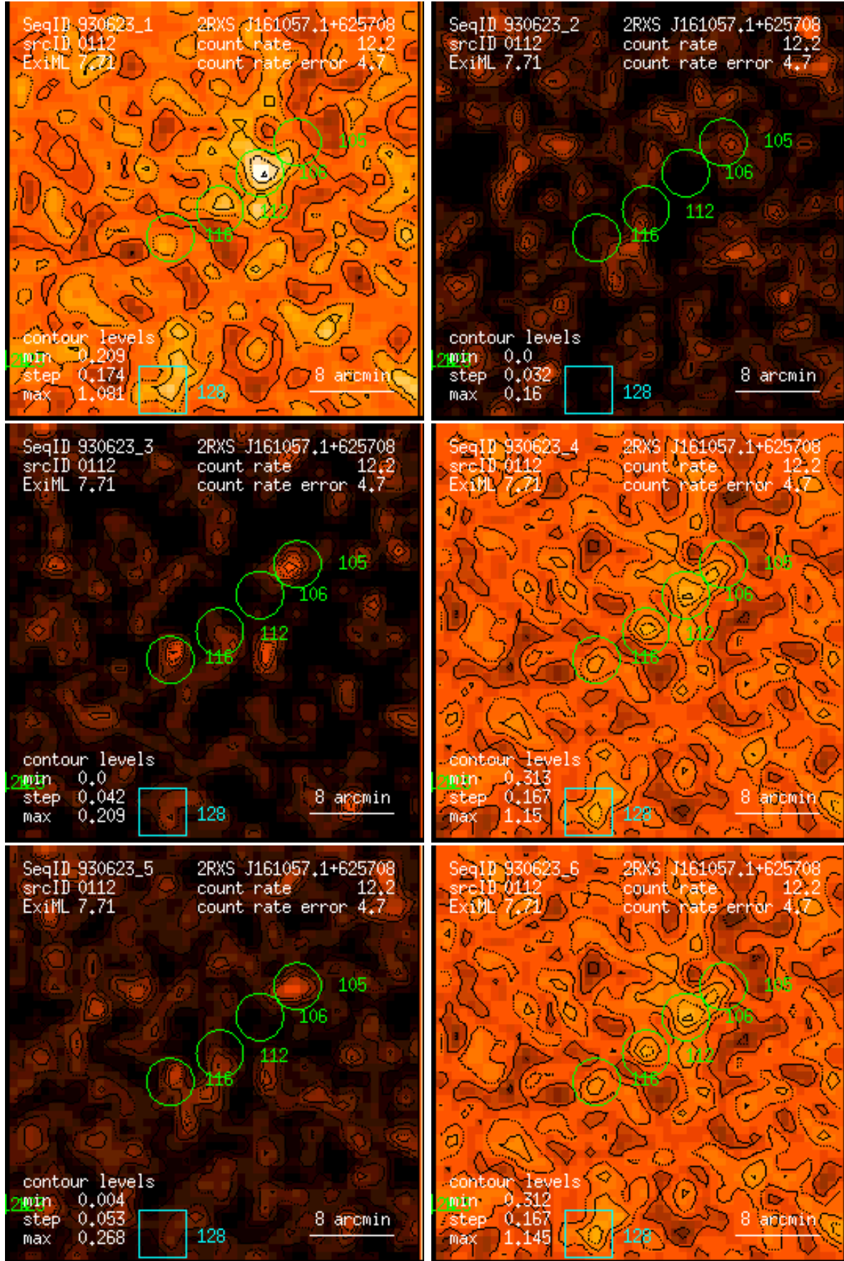
Figure 112: RASS 930623: detection 0112: band rate images, Gaussian filter: (1) PSPC channels 11 – 41, (2) 52 – 90, (3) 91 – 201, (4) 11 – 235, (5) 52 – 201, (6) 11 – 201. Broad band rates in counts/ks. Band rate contour levels in counts/ks/arcmin 2 .
