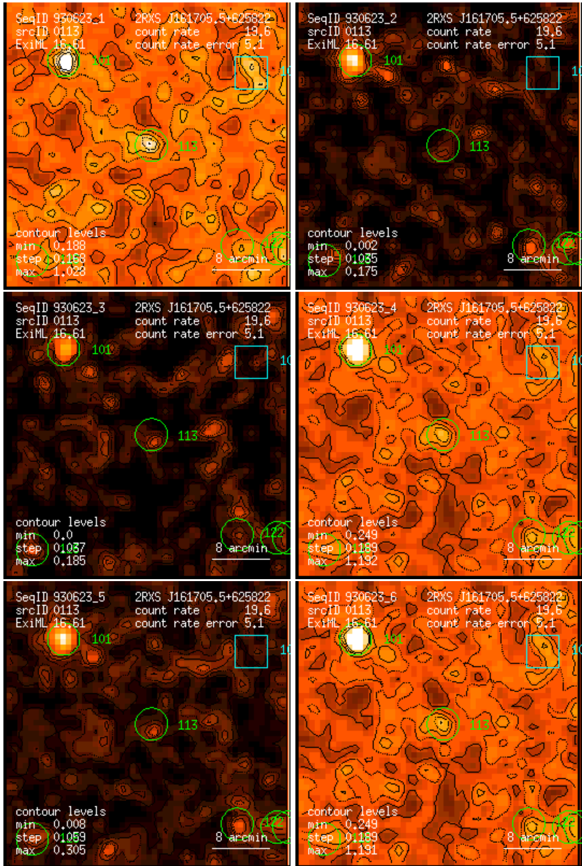
Figure 113: RASS 930623: detection 0113: band rate images, Gaussian filter: (1) PSPC channels 11 – 41, (2) 52 – 90, (3) 91 – 201, (4) 11 – 235, (5) 52 – 201, (6) 11 – 201. Broad band rates in counts/ks. Band rate contour levels in counts/ks/arcmin 2 .
