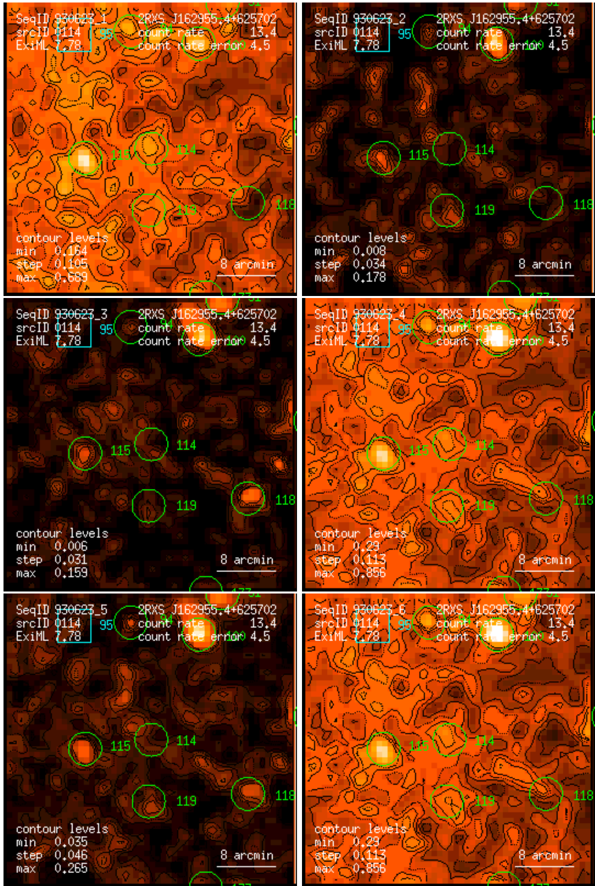
Figure 114: RASS 930623: detection 0114: band rate images, Gaussian filter: (1) PSPC channels 11 – 41, (2) 52 – 90, (3) 91 – 201, (4) 11 – 235, (5) 52 – 201, (6) 11 – 201. Broad band rates in counts/ks. Band rate contour levels in counts/ks/arcmin 2 .
