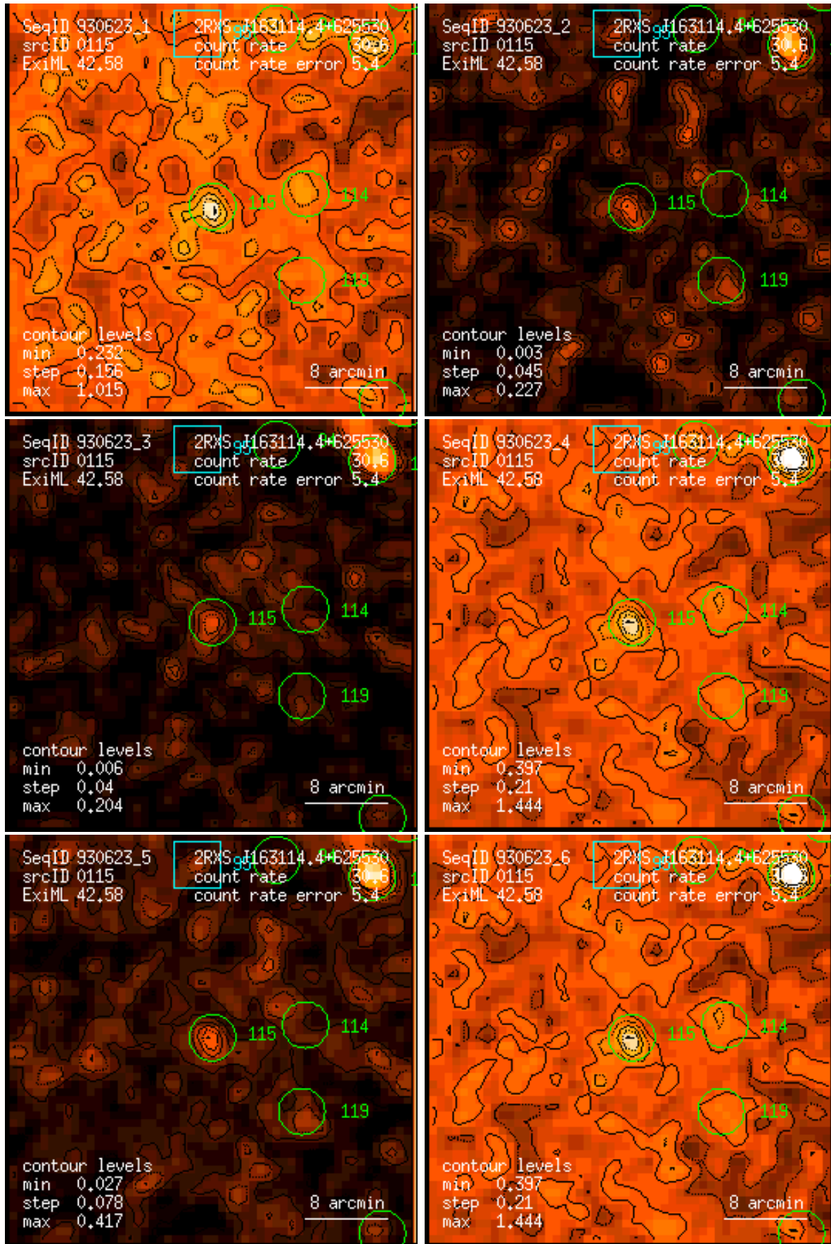
Figure 115: RASS 930623: detection 0115: band rate images, Gaussian filter: (1) PSPC channels 11 – 41, (2) 52 – 90, (3) 91 – 201, (4) 11 – 235, (5) 52 – 201, (6) 11 – 201. Broad band rates in counts/ks. Band rate contour levels in counts/ks/arcmin 2 .
