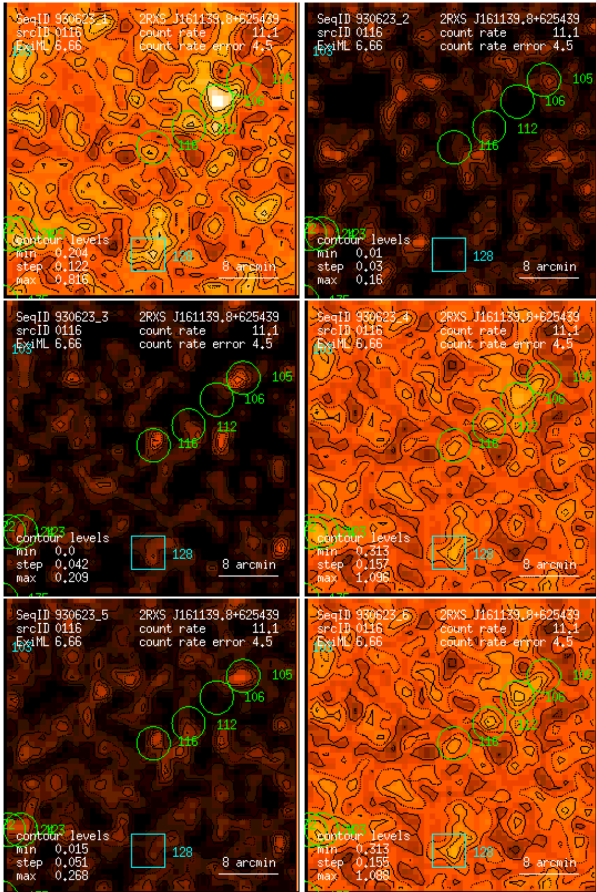
Figure 116: RASS 930623: detection 0116: band rate images, Gaussian filter: (1) PSPC channels 11 – 41, (2) 52 – 90, (3) 91 – 201, (4) 11 – 235, (5) 52 – 201, (6) 11 – 201. Broad band rates in counts/ks. Band rate contour levels in counts/ks/arcmin 2 .
