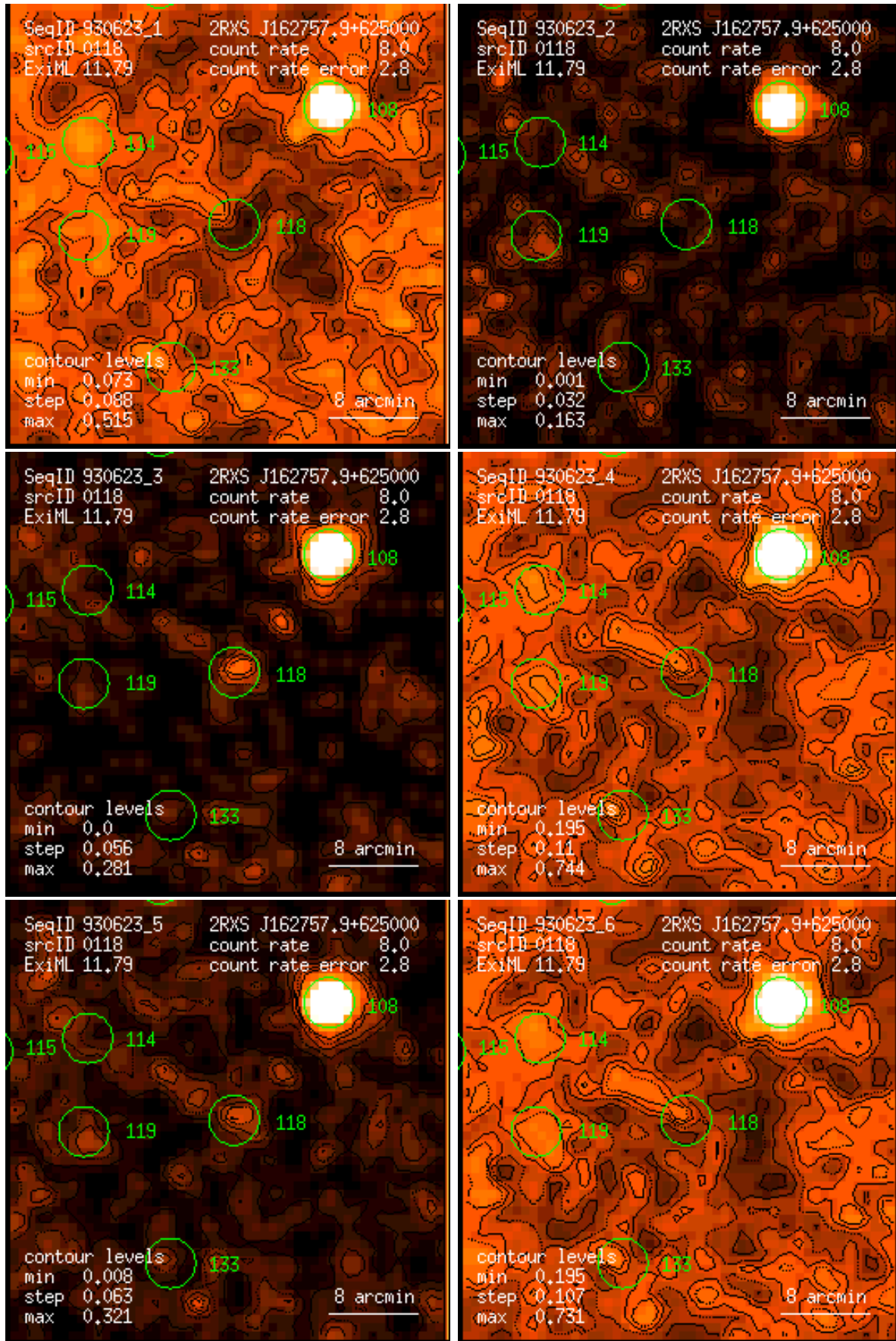
Figure 118: RASS 930623: detection 0118: band rate images, Gaussian filter: (1) PSPC channels 11 – 41, (2) 52 – 90, (3) 91 – 201, (4) 11 – 235, (5) 52 – 201, (6) 11 – 201. Broad band rates in counts/ks. Band rate contour levels in counts/ks/arcmin 2 .
