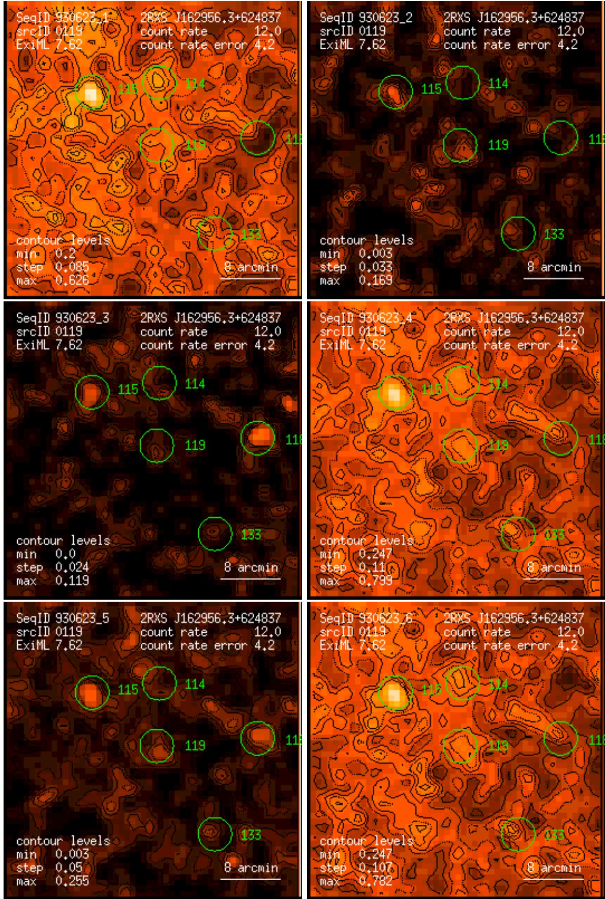
Figure 119: RASS 930623: detection 0119: band rate images, Gaussian filter: (1) PSPC channels 11 – 41, (2) 52 – 90, (3) 91 – 201, (4) 11 – 235, (5) 52 – 201, (6) 11 – 201. Broad band rates in counts/ks. Band rate contour levels in counts/ks/arcmin 2 .
