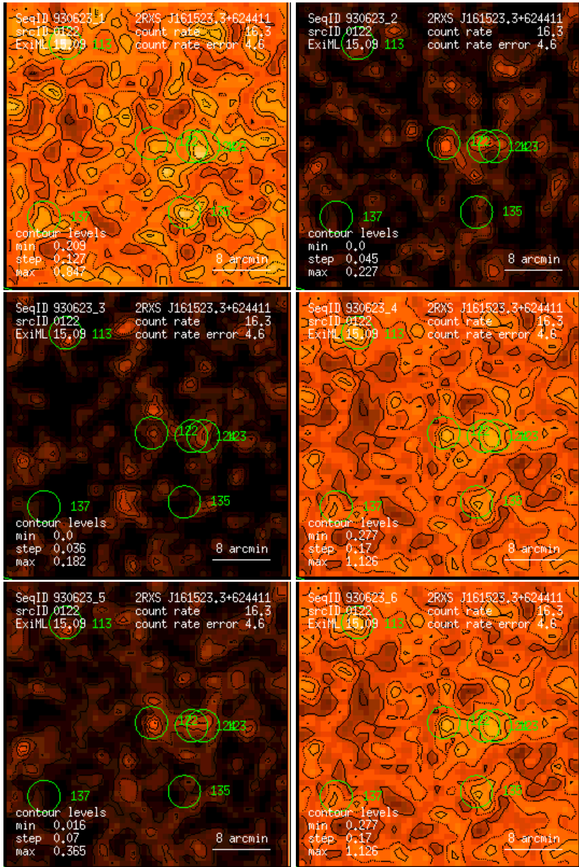
Figure 122: RASS 930623: detection 0122: band rate images, Gaussian filter: (1) PSPC channels 11 – 41, (2) 52 – 90, (3) 91 – 201, (4) 11 – 235, (5) 52 – 201, (6) 11 – 201. Broad band rates in counts/ks. Band rate contour levels in counts/ks/arcmin 2 .
