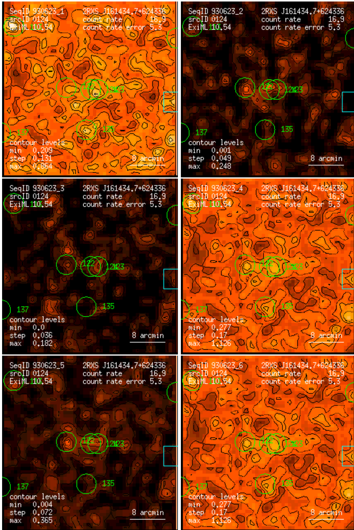
Figure 124: RASS 930623: detection 0124: band rate images, Gaussian filter: (1) PSPC channels 11 – 41, (2) 52 – 90, (3) 91 – 201, (4) 11 – 235, (5) 52 – 201, (6) 11 – 201. Broad band rates in counts/ks. Band rate contour levels in counts/ks/arcmin 2 .
