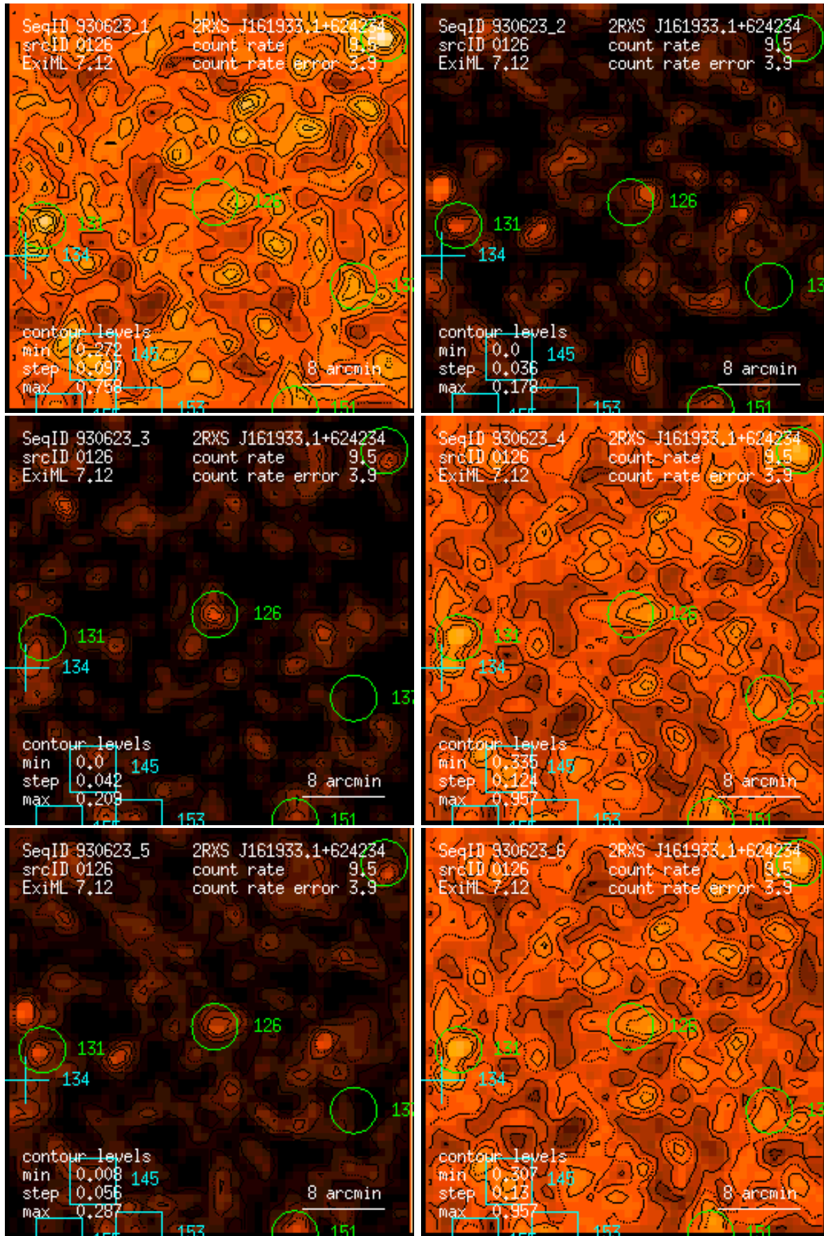
Figure 126: RASS 930623: detection 0126: band rate images, Gaussian filter: (1) PSPC channels 11 – 41, (2) 52 – 90, (3) 91 – 201, (4) 11 – 235, (5) 52 – 201, (6) 11 – 201. Broad band rates in counts/ks. Band rate contour levels in counts/ks/arcmin 2 .
