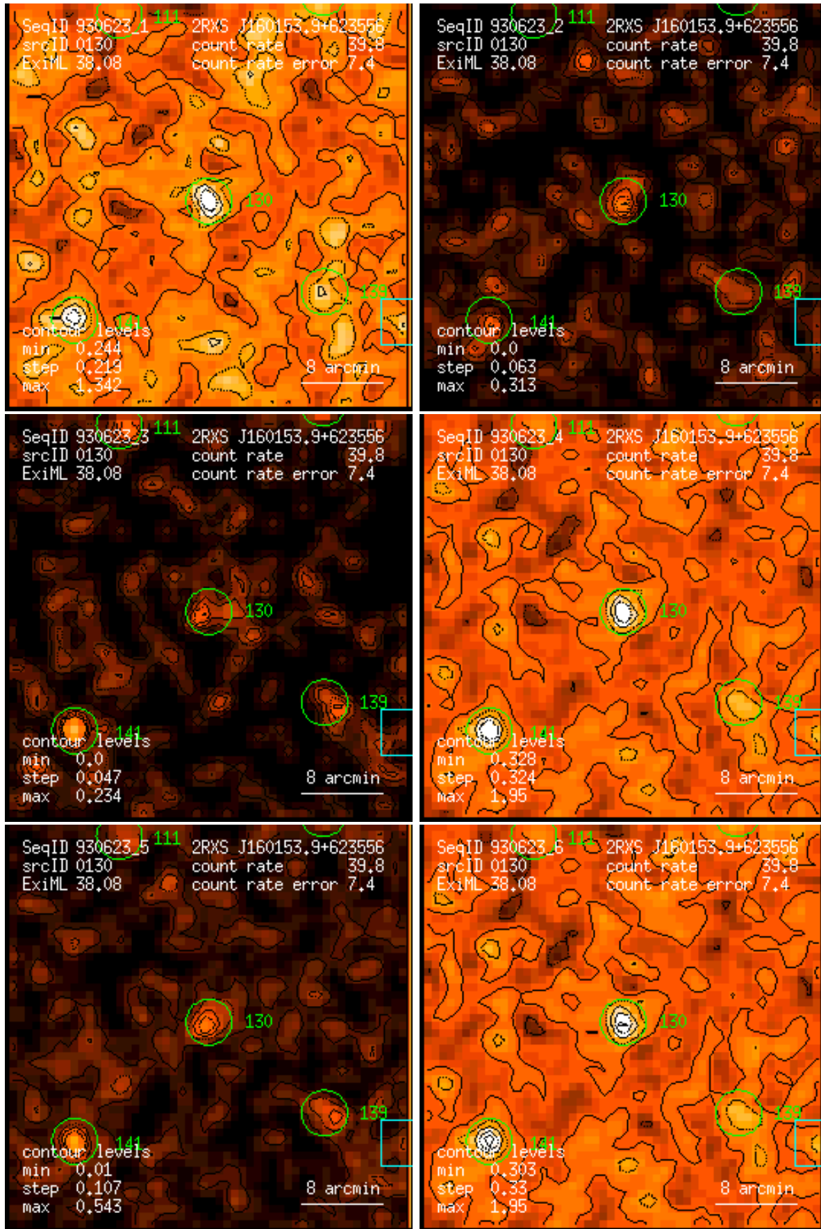
Figure 130: RASS 930623: detection 0130: band rate images, Gaussian filter: (1) PSPC channels 11 – 41, (2) 52 – 90, (3) 91 – 201, (4) 11 – 235, (5) 52 – 201, (6) 11 – 201. Broad band rates in counts/ks. Band rate contour levels in counts/ks/arcmin 2 .
