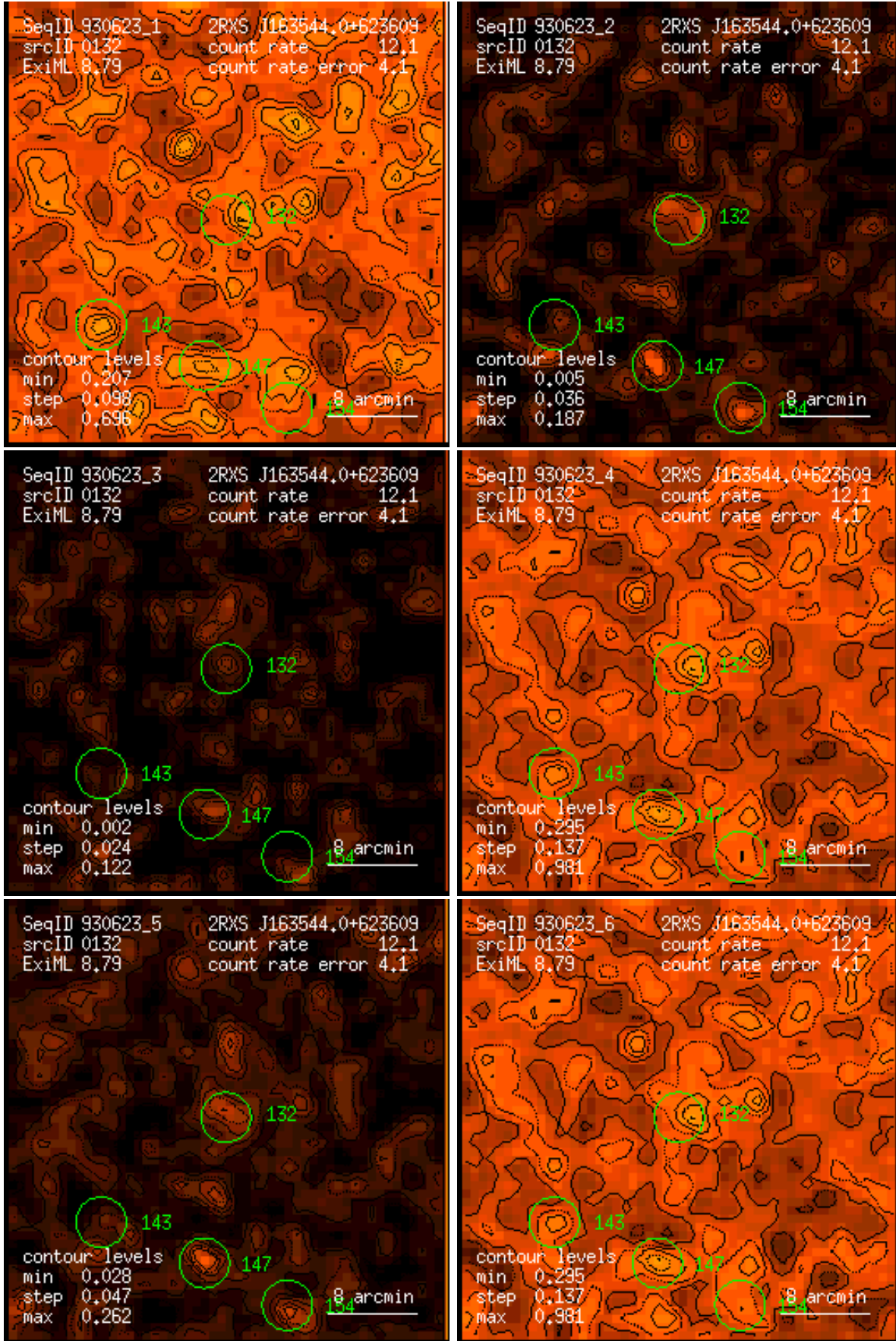
Figure 132: RASS 930623: detection 0132: band rate images, Gaussian filter: (1) PSPC channels 11 – 41, (2) 52 – 90, (3) 91 – 201, (4) 11 – 235, (5) 52 – 201, (6) 11 – 201. Broad band rates in counts/ks. Band rate contour levels in counts/ks/arcmin 2 .
