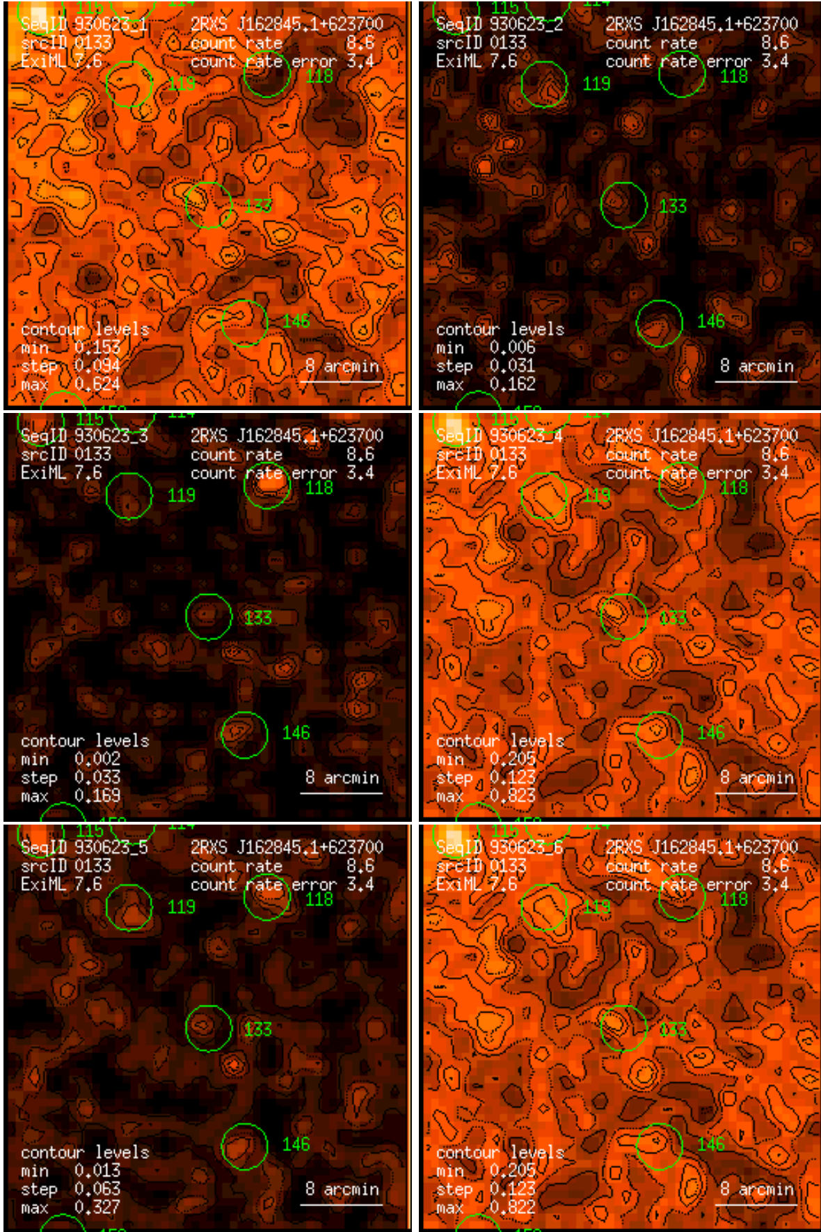
Figure 133: RASS 930623: detection 0133: band rate images, Gaussian filter: (1) PSPC channels 11 – 41, (2) 52 – 90, (3) 91 – 201, (4) 11 – 235, (5) 52 – 201, (6) 11 – 201. Broad band rates in counts/ks. Band rate contour levels in counts/ks/arcmin 2 .
