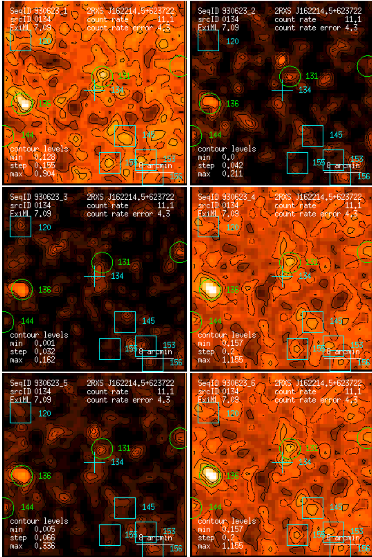
Figure 134: RASS 930623: detection 0134: band rate images, Gaussian filter: (1) PSPC channels 11 – 41, (2) 52 – 90, (3) 91 – 201, (4) 11 – 235, (5) 52 – 201, (6) 11 – 201. Broad band rates in counts/ks. Band rate contour levels in counts/ks/arcmin 2 .
