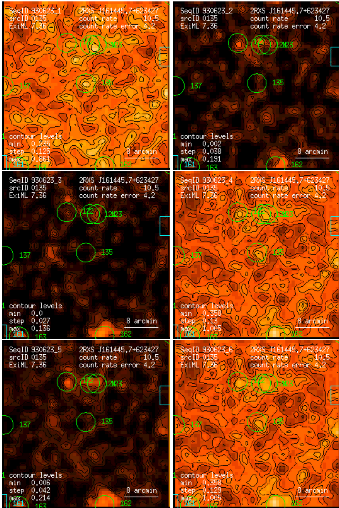
Figure 135: RASS 930623: detection 0135: band rate images, Gaussian filter: (1) PSPC channels 11 – 41, (2) 52 – 90, (3) 91 – 201, (4) 11 – 235, (5) 52 – 201, (6) 11 – 201. Broad band rates in counts/ks. Band rate contour levels in counts/ks/arcmin 2 .
