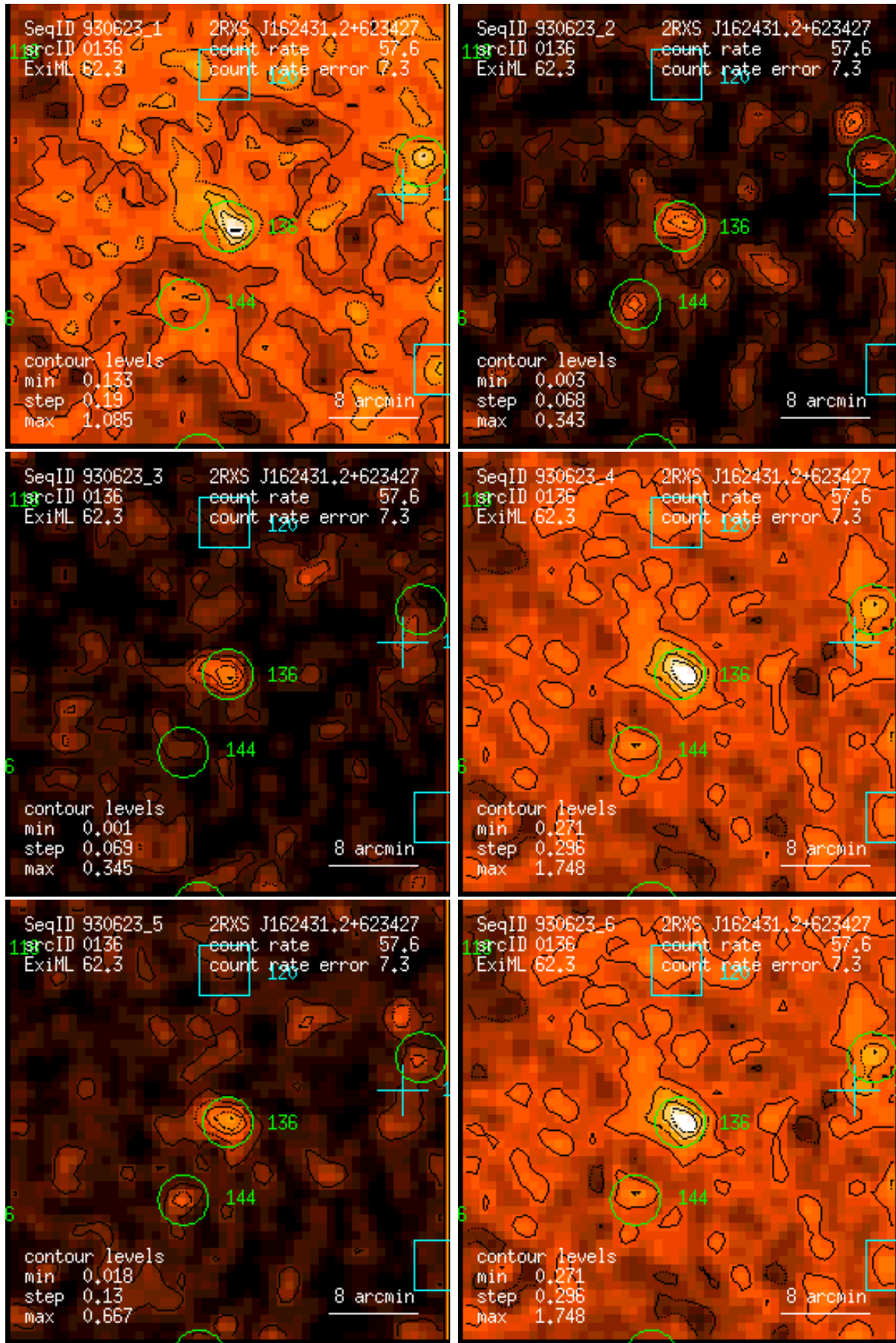
Figure 136: RASS 930623: detection 0136: band rate images, Gaussian filter: (1) PSPC channels 11 – 41, (2) 52 – 90, (3) 91 – 201, (4) 11 – 235, (5) 52 – 201, (6) 11 – 201. Broad band rates in counts/ks. Band rate contour levels in counts/ks/arcmin 2 .
