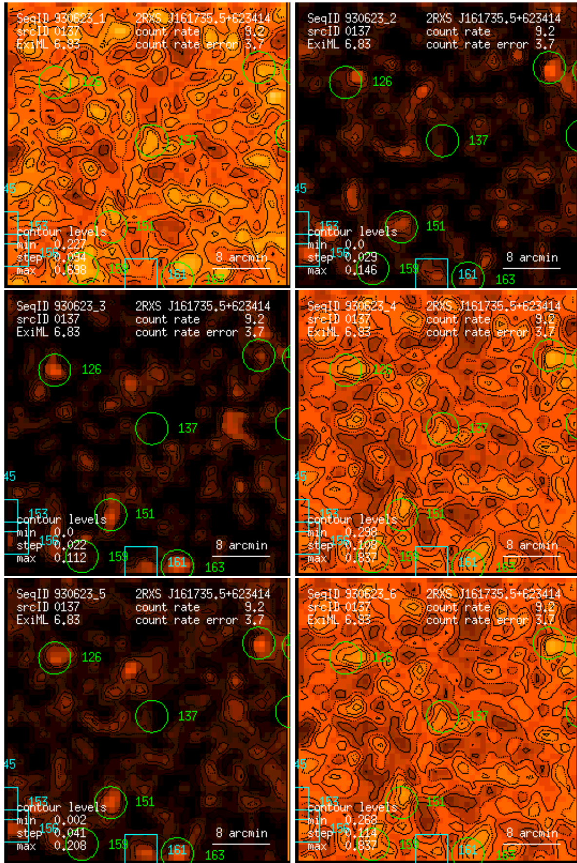
Figure 137: RASS 930623: detection 0137: band rate images, Gaussian filter: (1) PSPC channels 11 – 41, (2) 52 – 90, (3) 91 – 201, (4) 11 – 235, (5) 52 – 201, (6) 11 – 201. Broad band rates in counts/ks. Band rate contour levels in counts/ks/arcmin 2 .
