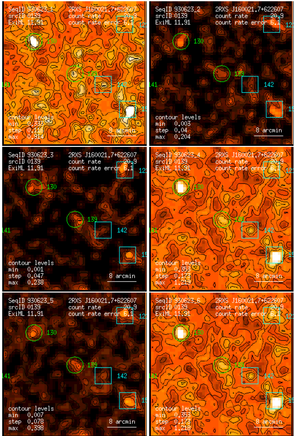
Figure 139: RASS 930623: detection 0139: band rate images, Gaussian filter: (1) PSPC channels 11 – 41, (2) 52 – 90, (3) 91 – 201, (4) 11 – 235, (5) 52 – 201, (6) 11 – 201. Broad band rates in counts/ks. Band rate contour levels in counts/ks/arcmin 2 .
