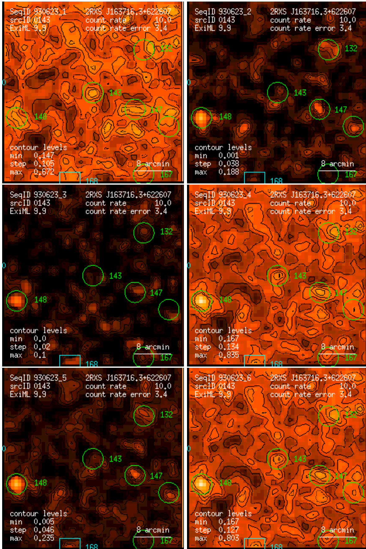
Figure 143: RASS 930623: detection 0143: band rate images, Gaussian filter: (1) PSPC channels 11 – 41, (2) 52 – 90, (3) 91 – 201, (4) 11 – 235, (5) 52 – 201, (6) 11 – 201. Broad band rates in counts/ks. Band rate contour levels in counts/ks/arcmin 2 .
