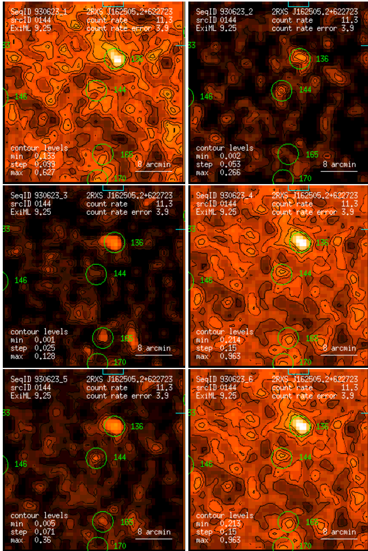
Figure 144: RASS 930623: detection 0144: band rate images, Gaussian filter: (1) PSPC channels 11 – 41, (2) 52 – 90, (3) 91 – 201, (4) 11 – 235, (5) 52 – 201, (6) 11 – 201. Broad band rates in counts/ks. Band rate contour levels in counts/ks/arcmin 2 .
