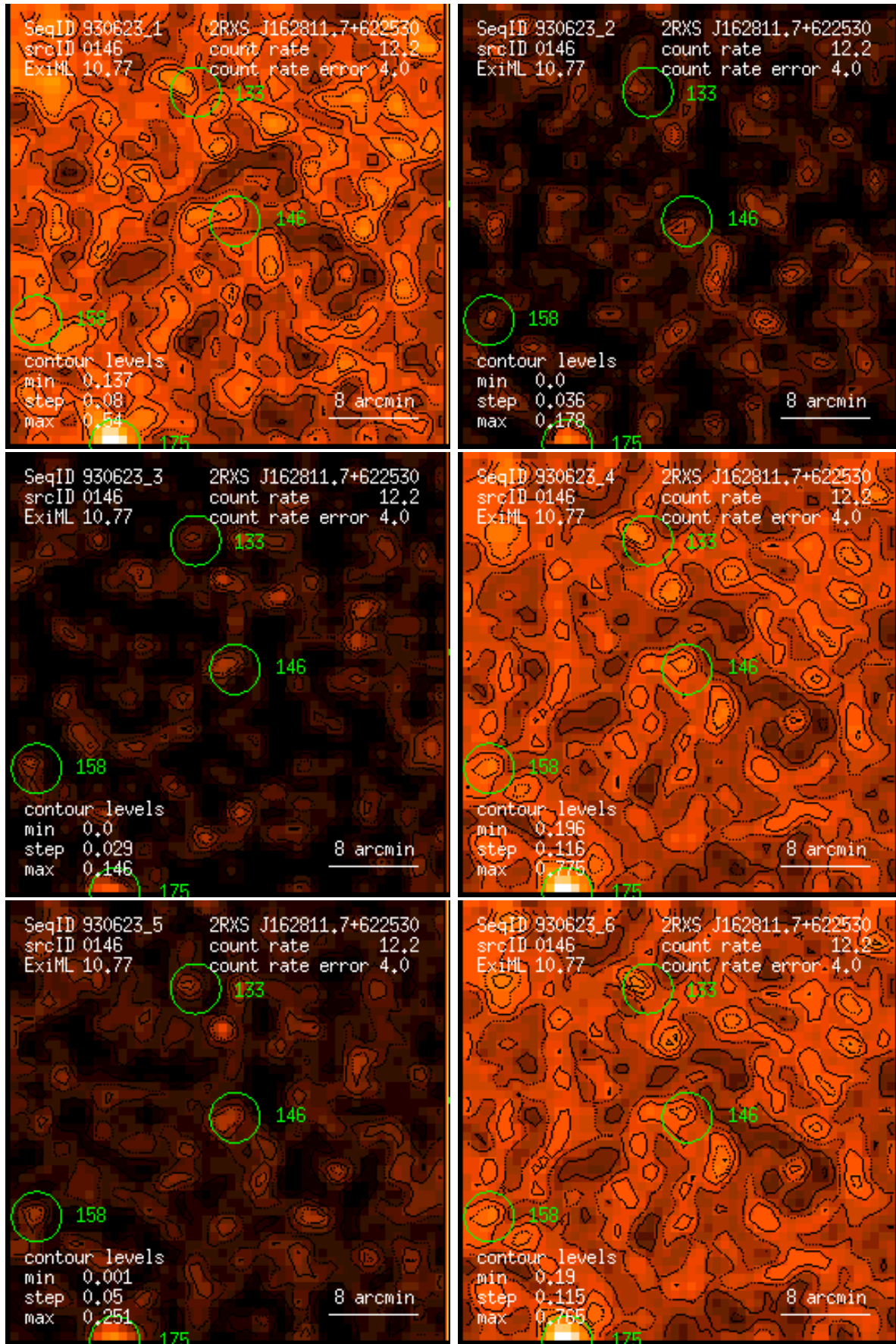
Figure 146: RASS 930623: detection 0146: band rate images, Gaussian filter: (1) PSPC channels 11 – 41, (2) 52 – 90, (3) 91 – 201, (4) 11 – 235, (5) 52 – 201, (6) 11 – 201. Broad band rates in counts/ks. Band rate contour levels in counts/ks/arcmin 2 .
