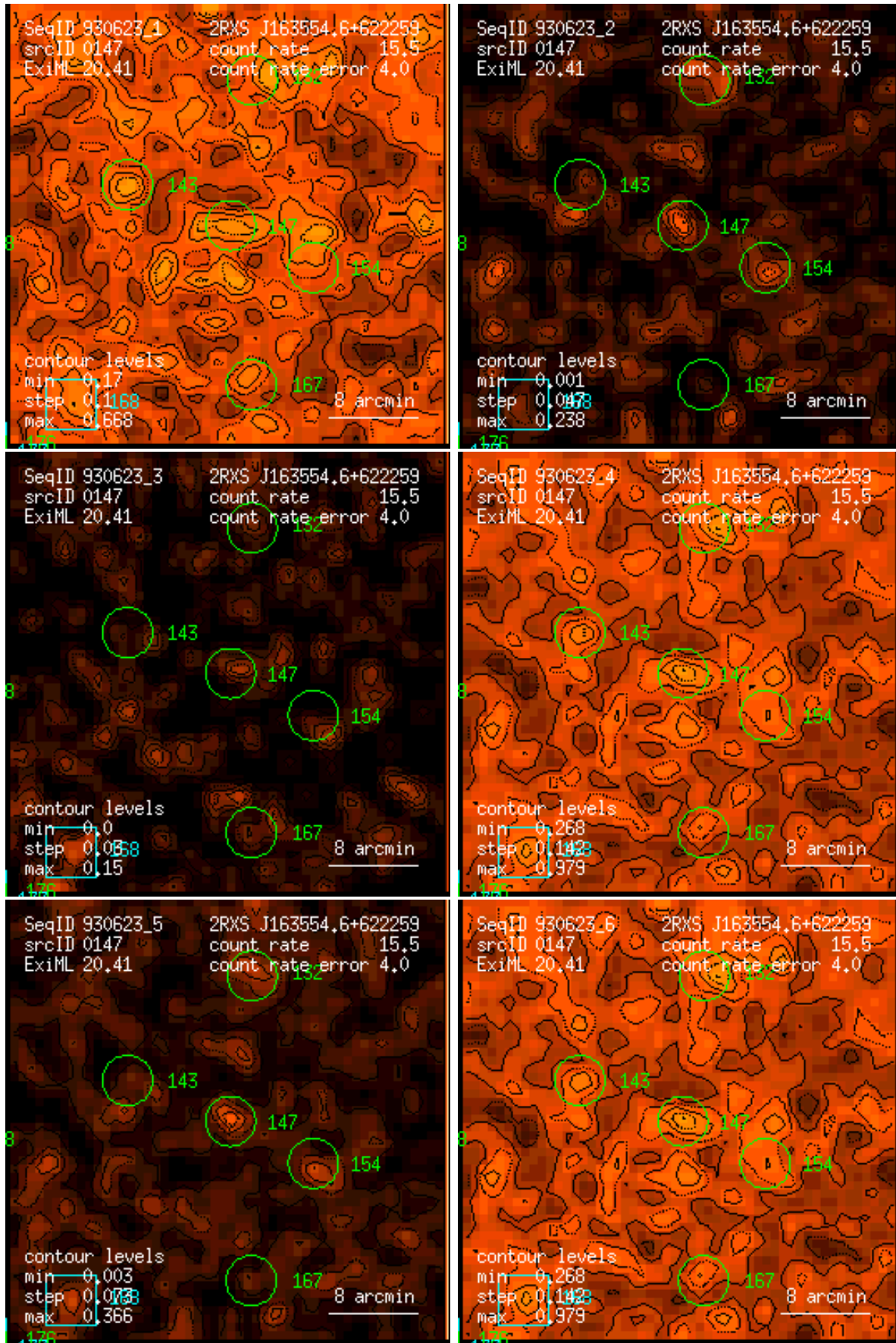
Figure 147: RASS 930623: detection 0147: band rate images, Gaussian filter: (1) PSPC channels 11 – 41, (2) 52 – 90, (3) 91 – 201, (4) 11 – 235, (5) 52 – 201, (6) 11 – 201. Broad band rates in counts/ks. Band rate contour levels in counts/ks/arcmin 2 .
