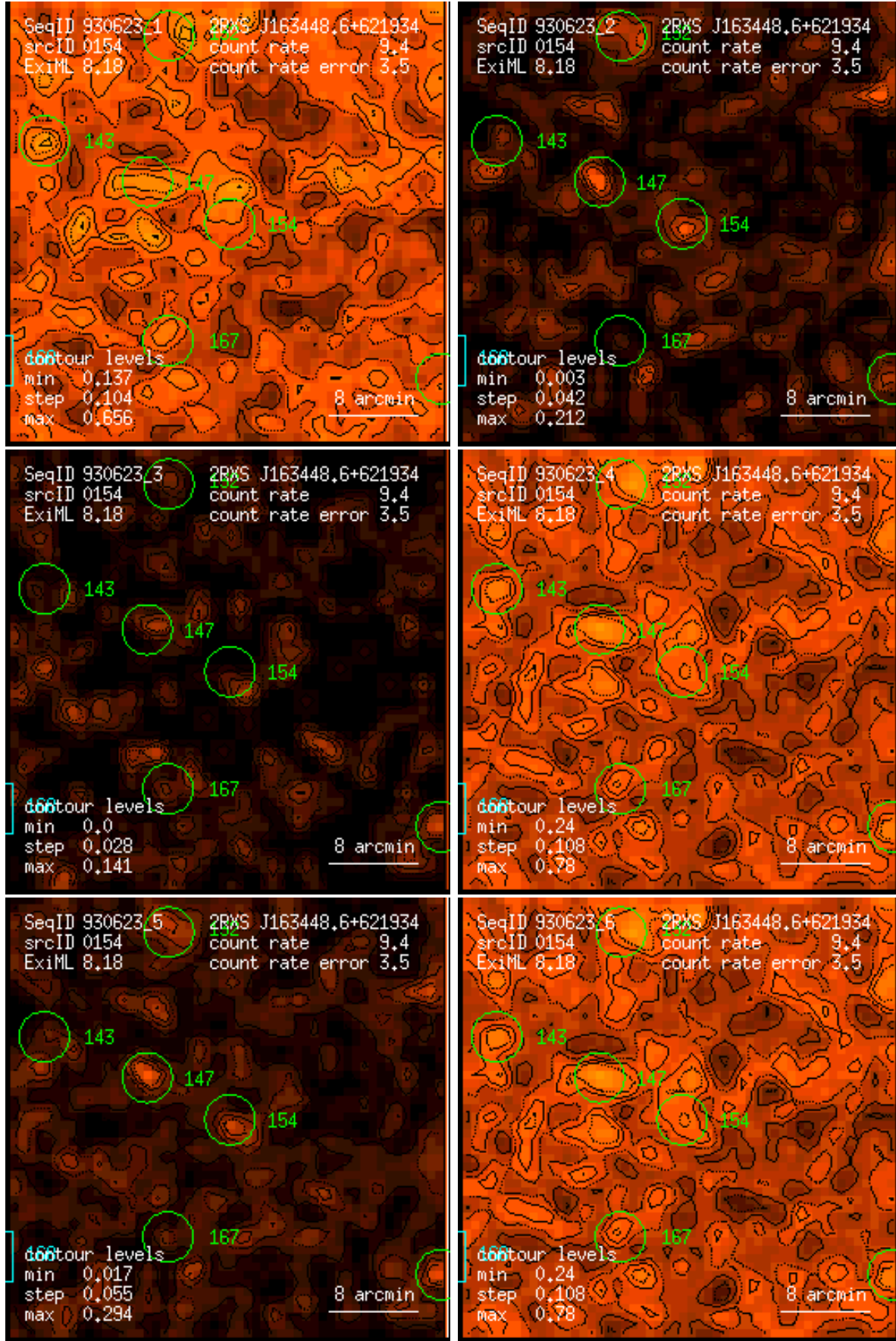
Figure 154: RASS 930623: detection 0154: band rate images, Gaussian filter: (1) PSPC channels 11 – 41, (2) 52 – 90, (3) 91 – 201, (4) 11 – 235, (5) 52 – 201, (6) 11 – 201. Broad band rates in counts/ks. Band rate contour levels in counts/ks/arcmin 2 .
