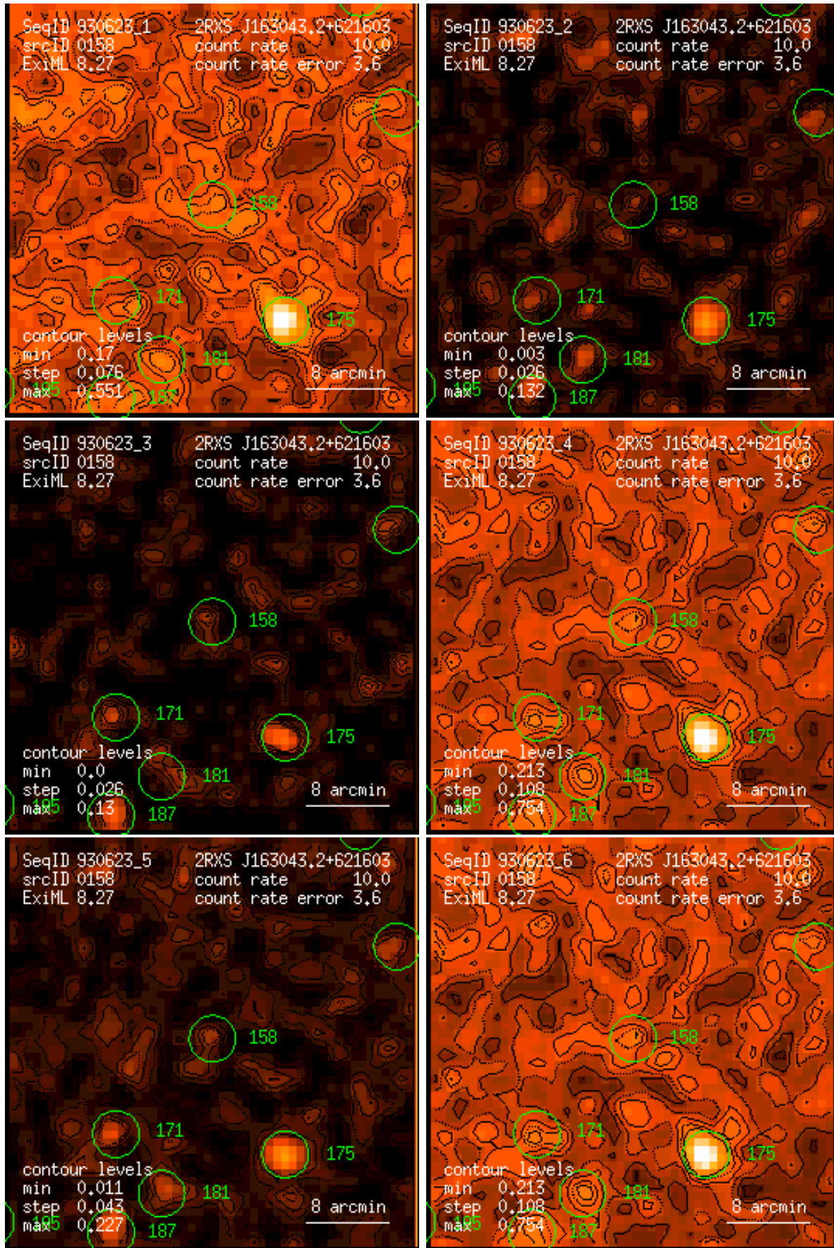
Figure 158: RASS 930623: detection 0158: band rate images, Gaussian filter: (1) PSPC channels 11 – 41, (2) 52 – 90, (3) 91 – 201, (4) 11 – 235, (5) 52 – 201, (6) 11 – 201. Broad band rates in counts/ks. Band rate contour levels in counts/ks/arcmin 2 .
