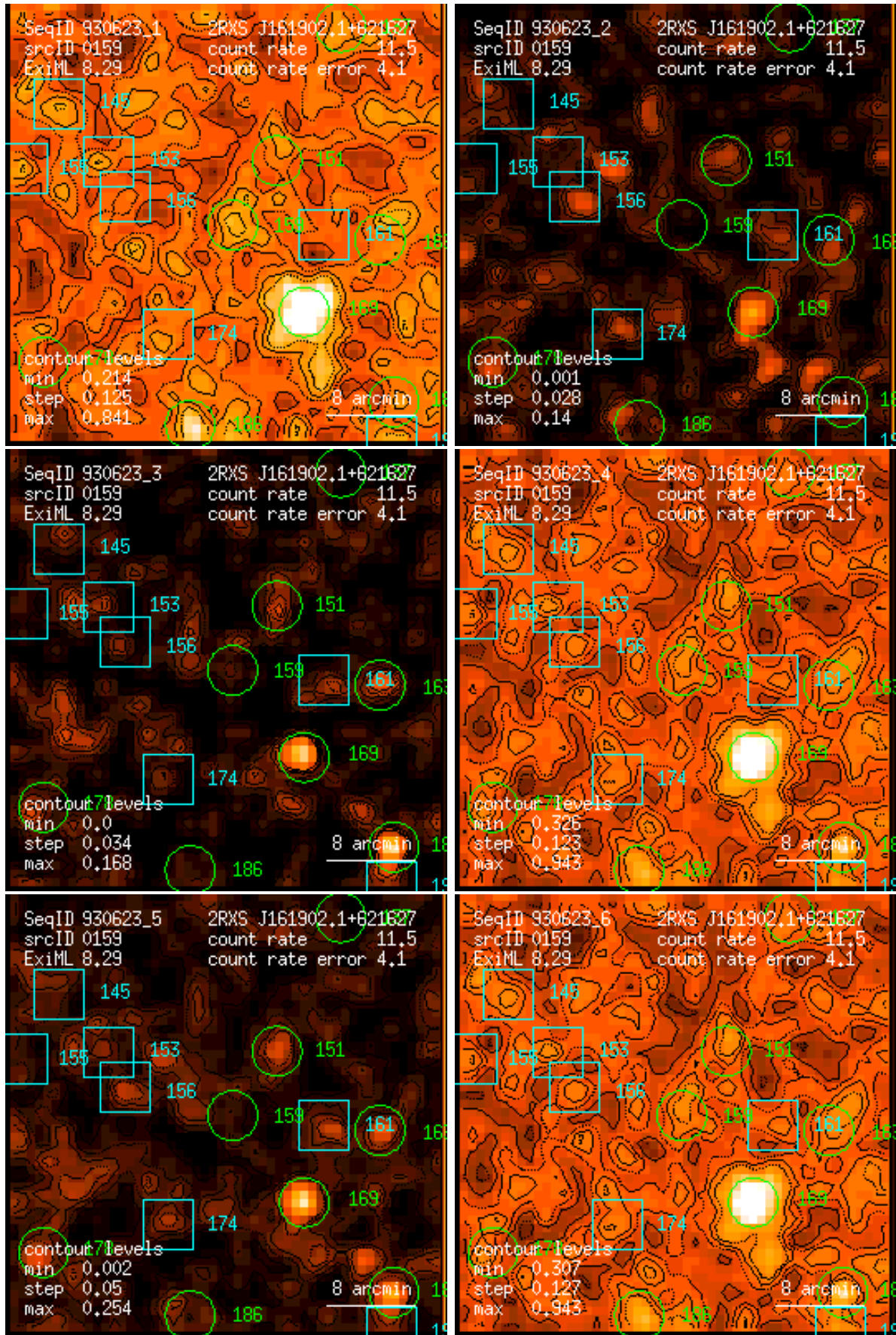
Figure 159: RASS 930623: detection 0159: band rate images, Gaussian filter: (1) PSPC channels 11 – 41, (2) 52 – 90, (3) 91 – 201, (4) 11 – 235, (5) 52 – 201, (6) 11 – 201. Broad band rates in counts/ks. Band rate contour levels in counts/ks/arcmin 2 .
