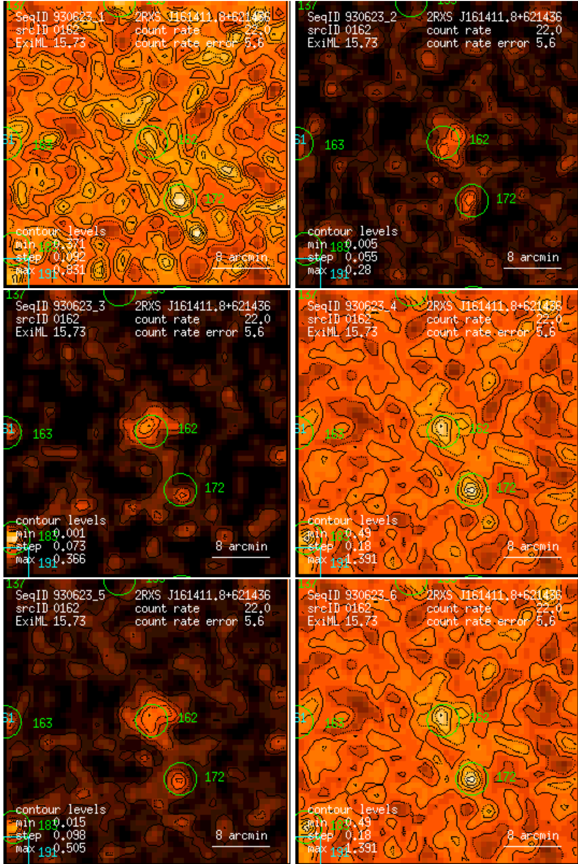
Figure 162: RASS 930623: detection 0162: band rate images, Gaussian filter: (1) PSPC channels 11 – 41, (2) 52 – 90, (3) 91 – 201, (4) 11 – 235, (5) 52 – 201, (6) 11 – 201. Broad band rates in counts/ks. Band rate contour levels in counts/ks/arcmin 2 .
