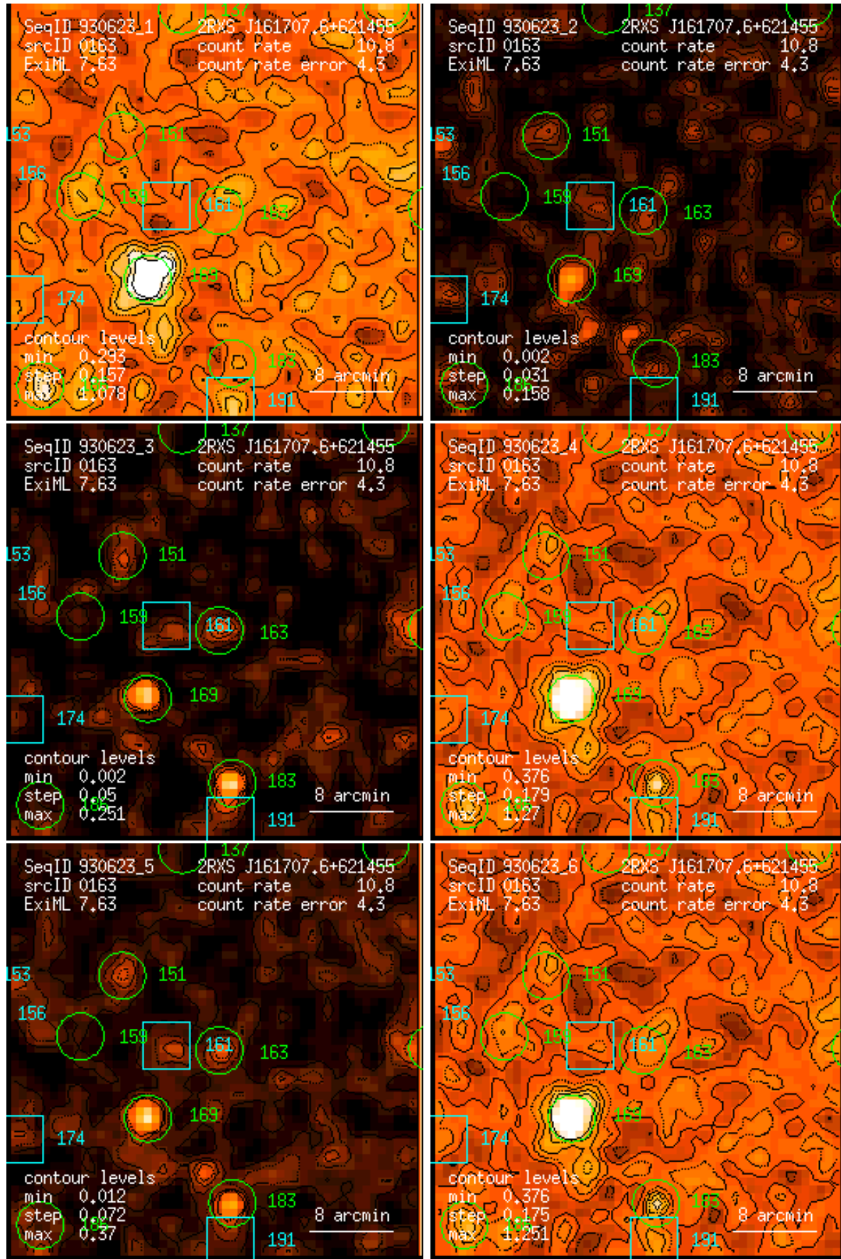
Figure 163: RASS 930623: detection 0163: band rate images, Gaussian filter: (1) PSPC channels 11 – 41, (2) 52 – 90, (3) 91 – 201, (4) 11 – 235, (5) 52 – 201, (6) 11 – 201. Broad band rates in counts/ks. Band rate contour levels in counts/ks/arcmin 2 .
