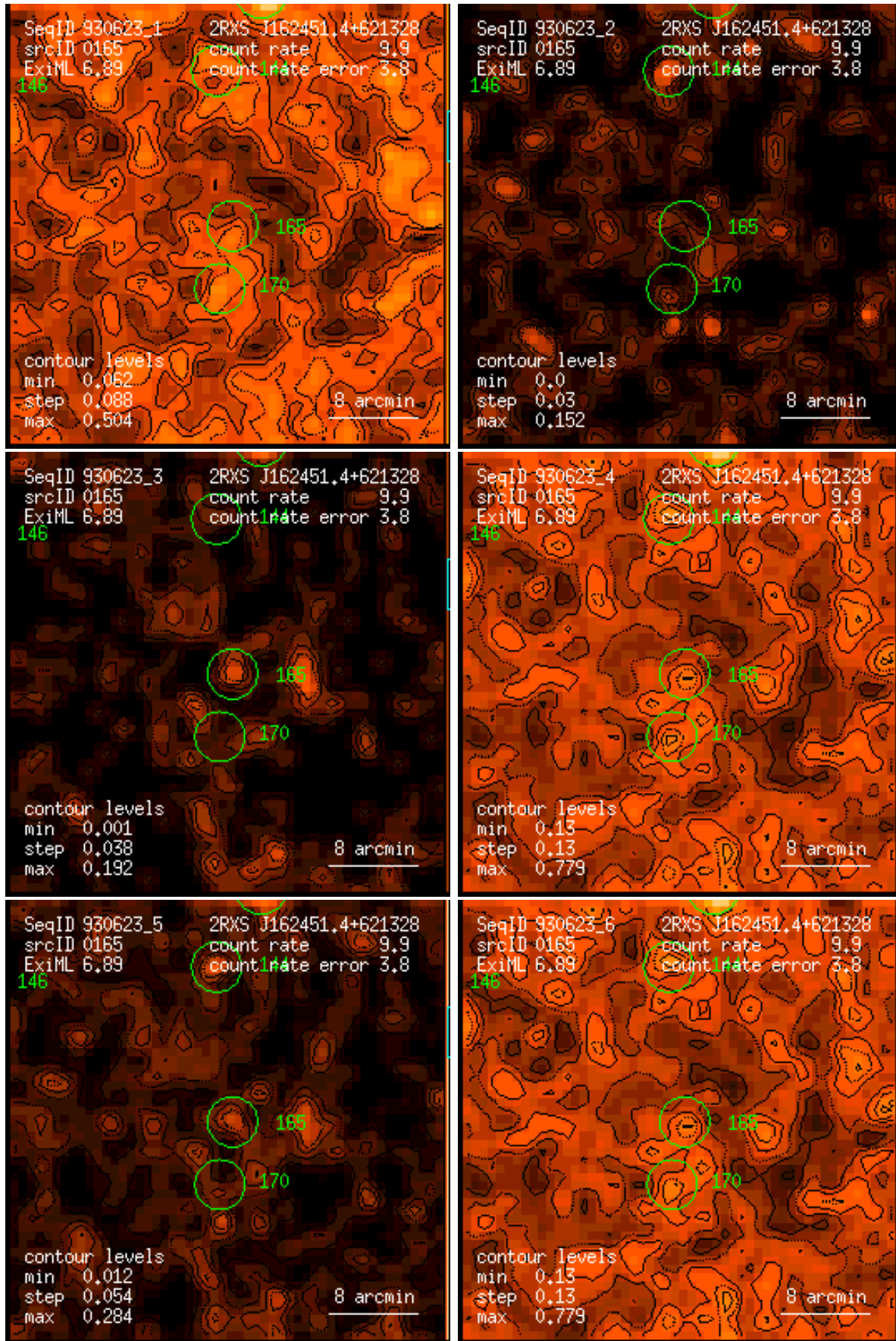
Figure 165: RASS 930623: detection 0165: band rate images, Gaussian filter: (1) PSPC channels 11 – 41, (2) 52 – 90, (3) 91 – 201, (4) 11 – 235, (5) 52 – 201, (6) 11 – 201. Broad band rates in counts/ks. Band rate contour levels in counts/ks/arcmin 2 .
