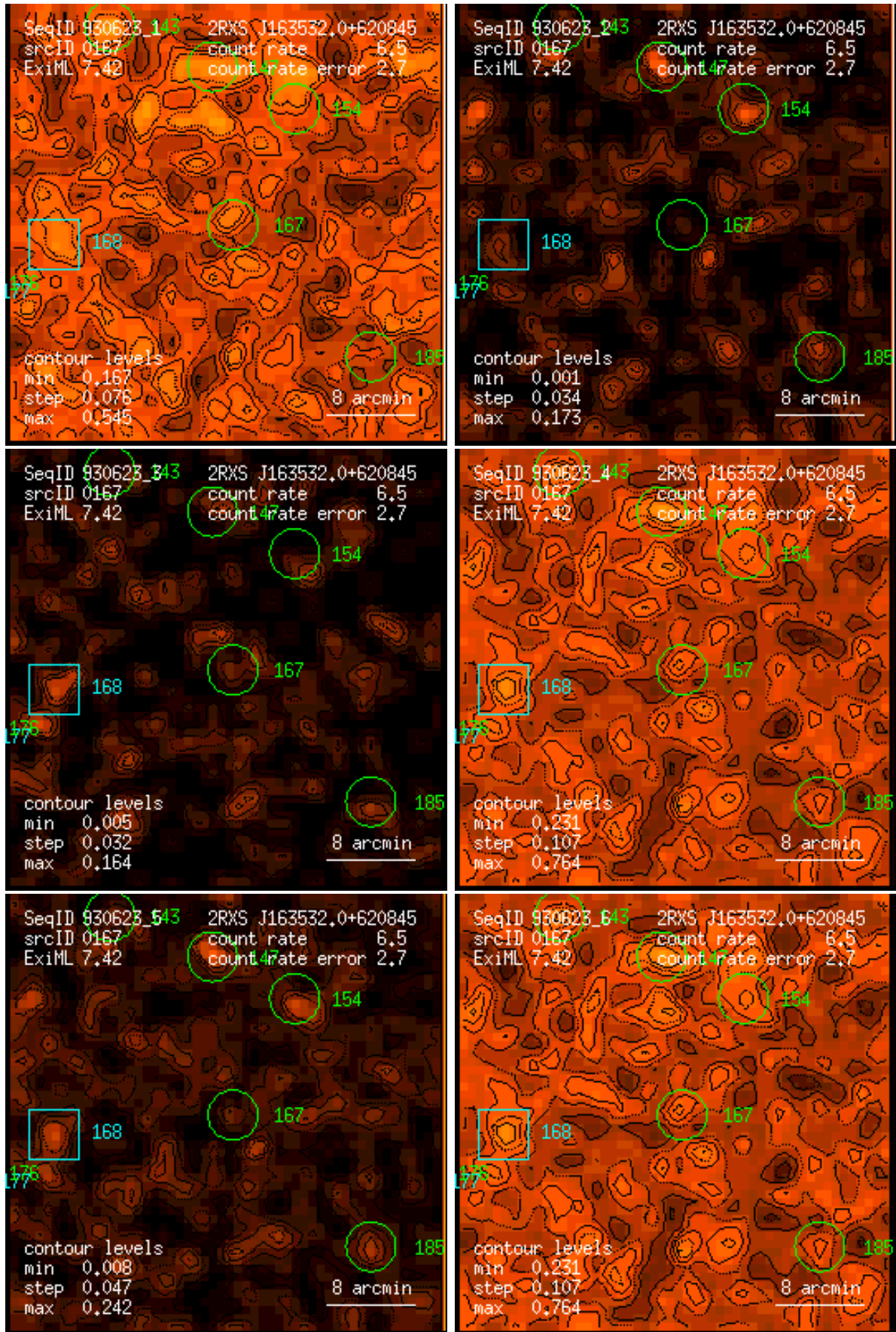
Figure 167: RASS 930623: detection 0167: band rate images, Gaussian filter: (1) PSPC channels 11 – 41, (2) 52 – 90, (3) 91 – 201, (4) 11 – 235, (5) 52 – 201, (6) 11 – 201. Broad band rates in counts/ks. Band rate contour levels in counts/ks/arcmin 2 .
