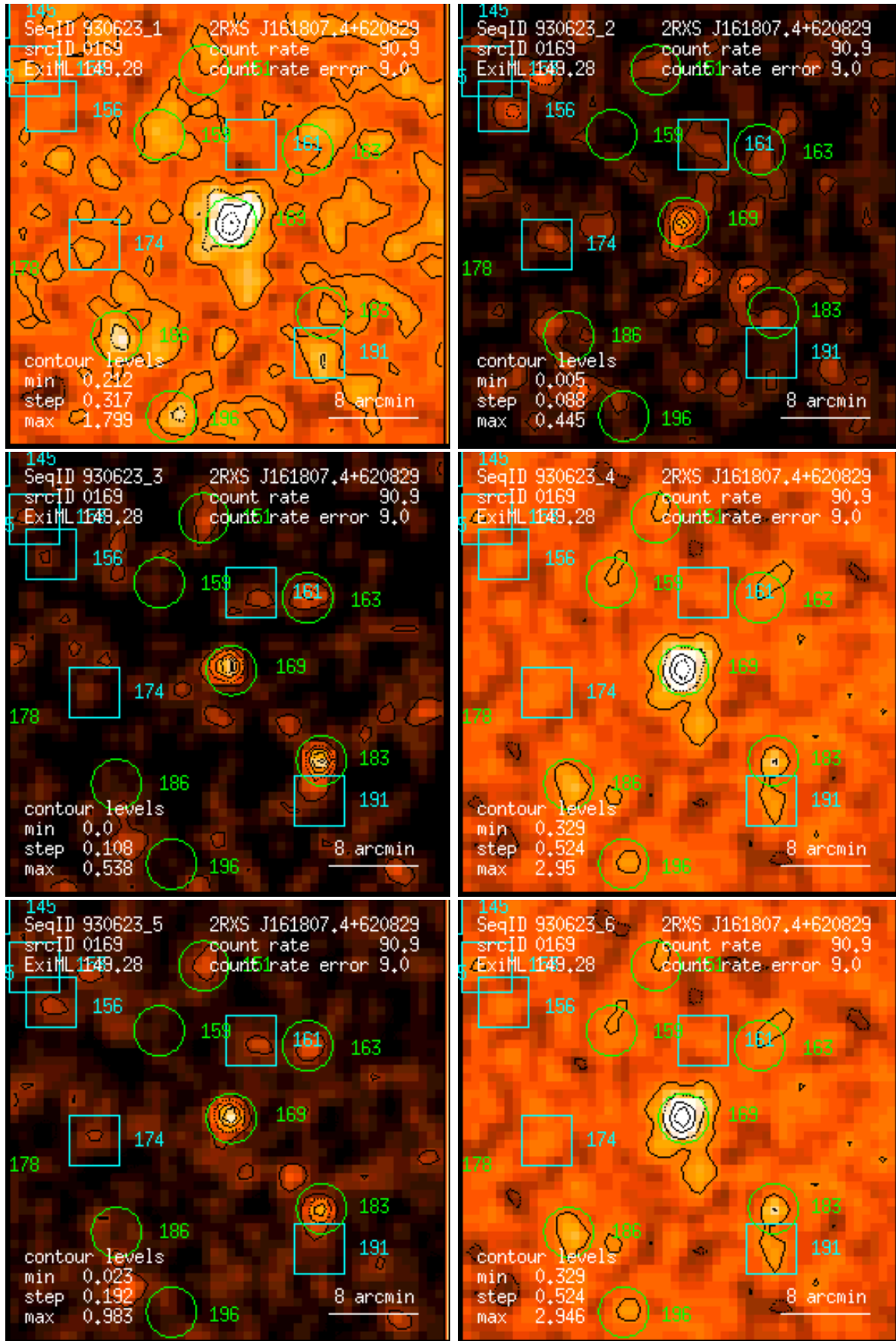
Figure 169: RASS 930623: detection 0169: band rate images, Gaussian filter: (1) PSPC channels 11 – 41, (2) 52 – 90, (3) 91 – 201, (4) 11 – 235, (5) 52 – 201, (6) 11 – 201. Broad band rates in counts/ks. Band rate contour levels in counts/ks/arcmin 2 .
