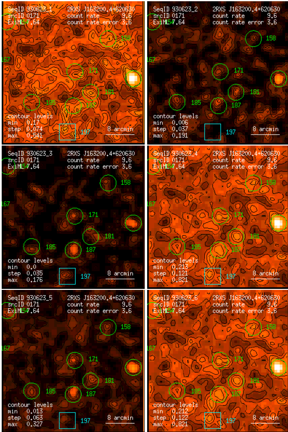
Figure 171: RASS 930623: detection 0171: band rate images, Gaussian filter: (1) PSPC channels 11 – 41, (2) 52 – 90, (3) 91 – 201, (4) 11 – 235, (5) 52 – 201, (6) 11 – 201. Broad band rates in counts/ks. Band rate contour levels in counts/ks/arcmin 2 .
