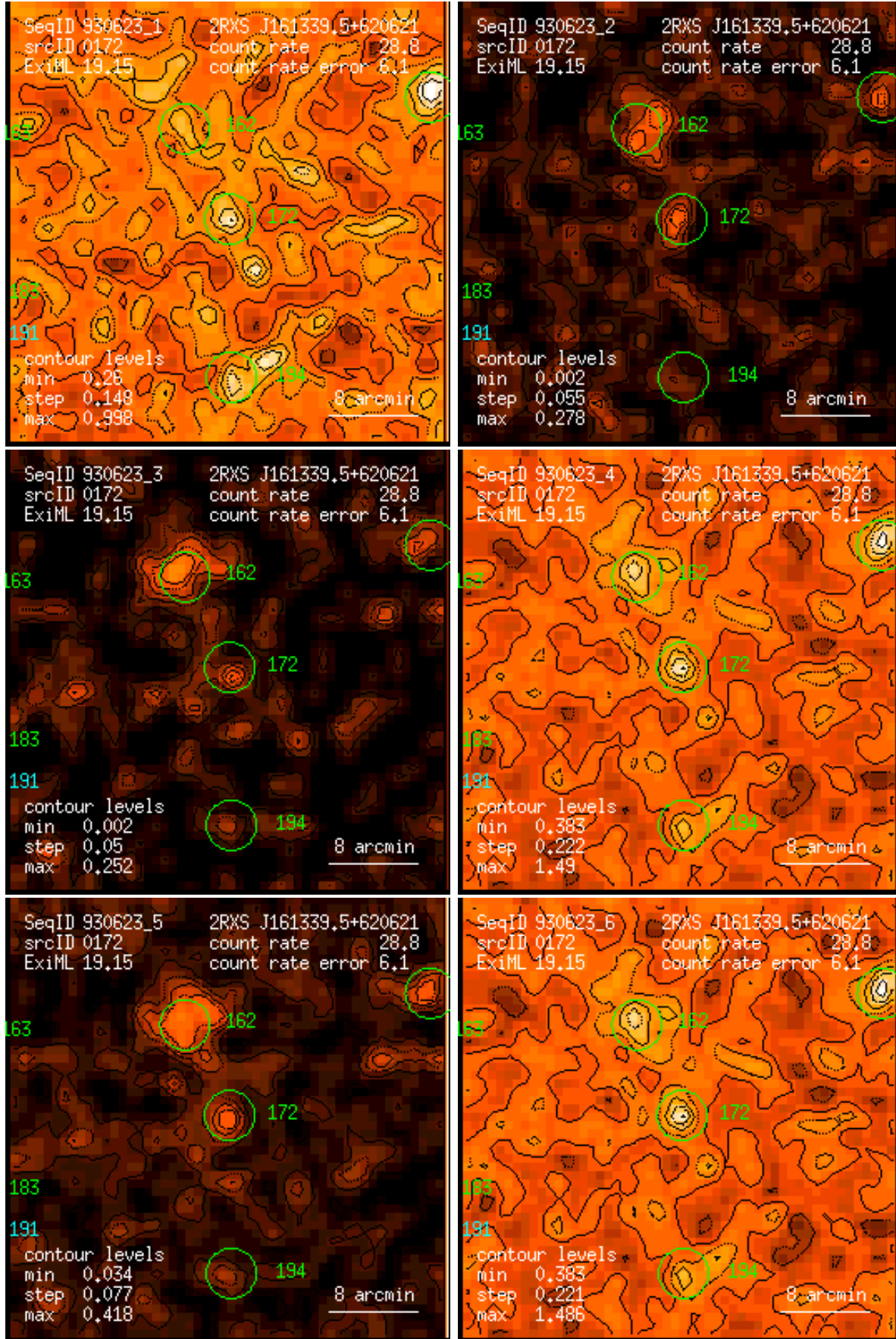
Figure 172: RASS 930623: detection 0172: band rate images, Gaussian filter: (1) PSPC channels 11 – 41, (2) 52 – 90, (3) 91 – 201, (4) 11 – 235, (5) 52 – 201, (6) 11 – 201. Broad band rates in counts/ks. Band rate contour levels in counts/ks/arcmin 2 .
