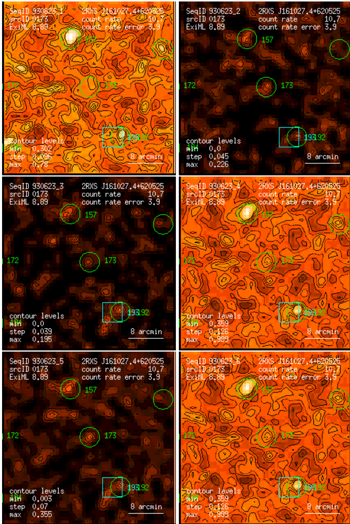
Figure 173: RASS 930623: detection 0173: band rate images, Gaussian filter: (1) PSPC channels 11 – 41, (2) 52 – 90, (3) 91 – 201, (4) 11 – 235, (5) 52 – 201, (6) 11 – 201. Broad band rates in counts/ks. Band rate contour levels in counts/ks/arcmin 2 .
