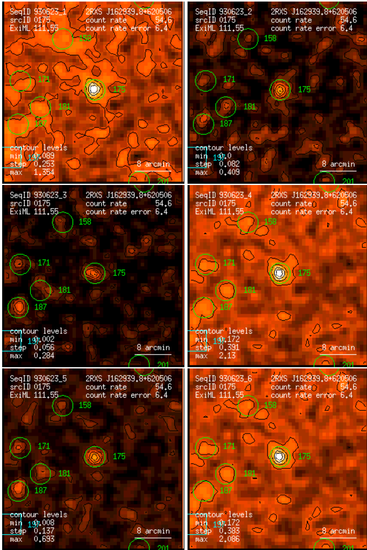
Figure 175: RASS 930623: detection 0175: band rate images, Gaussian filter: (1) PSPC channels 11 – 41, (2) 52 – 90, (3) 91 – 201, (4) 11 – 235, (5) 52 – 201, (6) 11 – 201. Broad band rates in counts/ks. Band rate contour levels in counts/ks/arcmin 2 .
