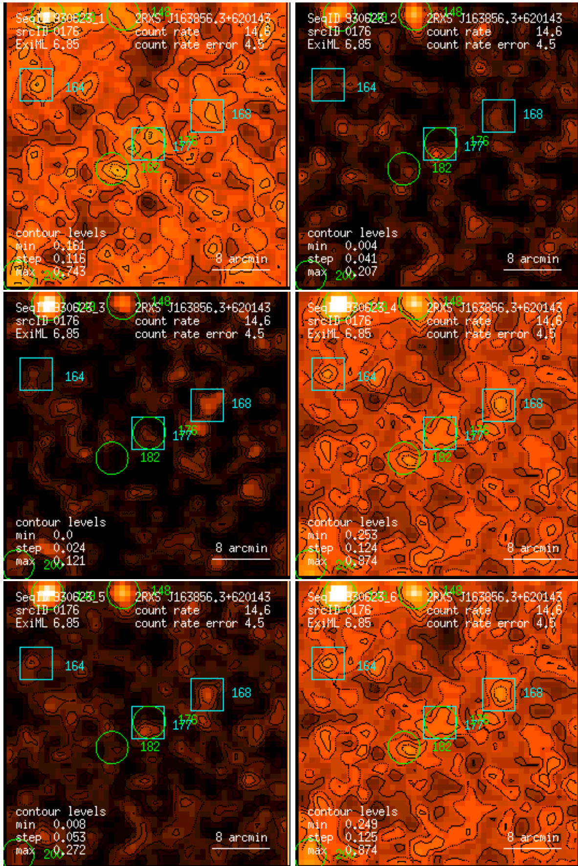
Figure 176: RASS 930623: detection 0176: band rate images, Gaussian filter: (1) PSPC channels 11 – 41, (2) 52 – 90, (3) 91 – 201, (4) 11 – 235, (5) 52 – 201, (6) 11 – 201. Broad band rates in counts/ks. Band rate contour levels in counts/ks/arcmin 2 .
