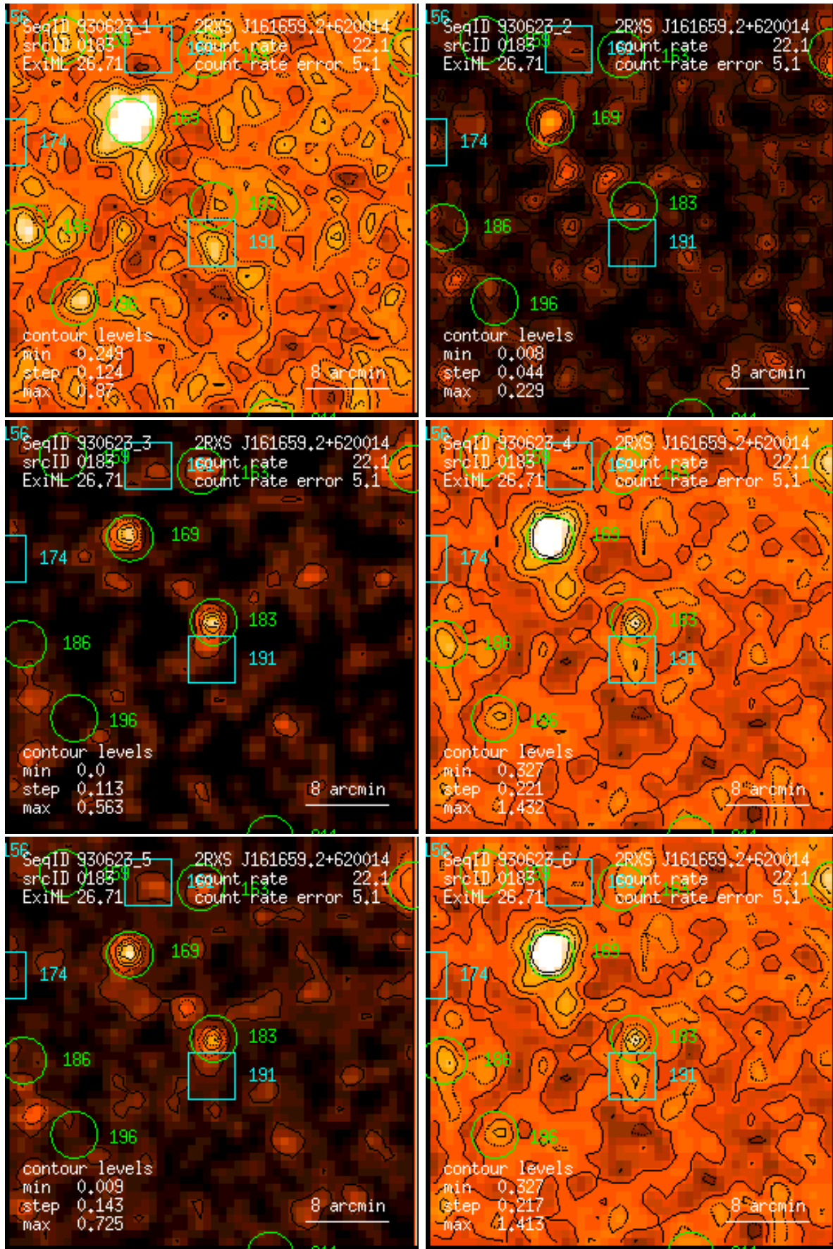
Figure 183: RASS 930623: detection 0183: band rate images, Gaussian filter: (1) PSPC channels 11 – 41, (2) 52 – 90, (3) 91 – 201, (4) 11 – 235, (5) 52 – 201, (6) 11 – 201. Broad band rates in counts/ks. Band rate contour levels in counts/ks/arcmin 2 .
