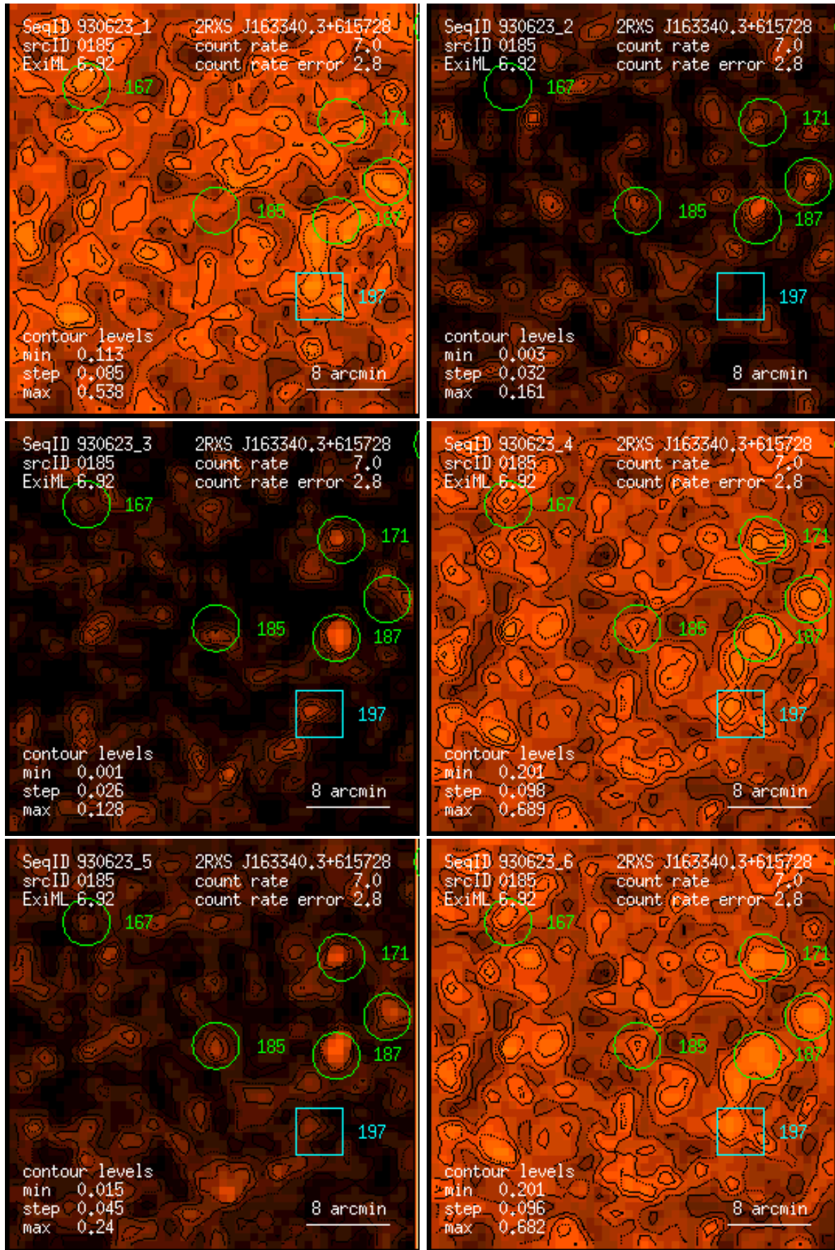
Figure 185: RASS 930623: detection 0185: band rate images, Gaussian filter: (1) PSPC channels 11 – 41, (2) 52 – 90, (3) 91 – 201, (4) 11 – 235, (5) 52 – 201, (6) 11 – 201. Broad band rates in counts/ks. Band rate contour levels in counts/ks/arcmin 2 .
