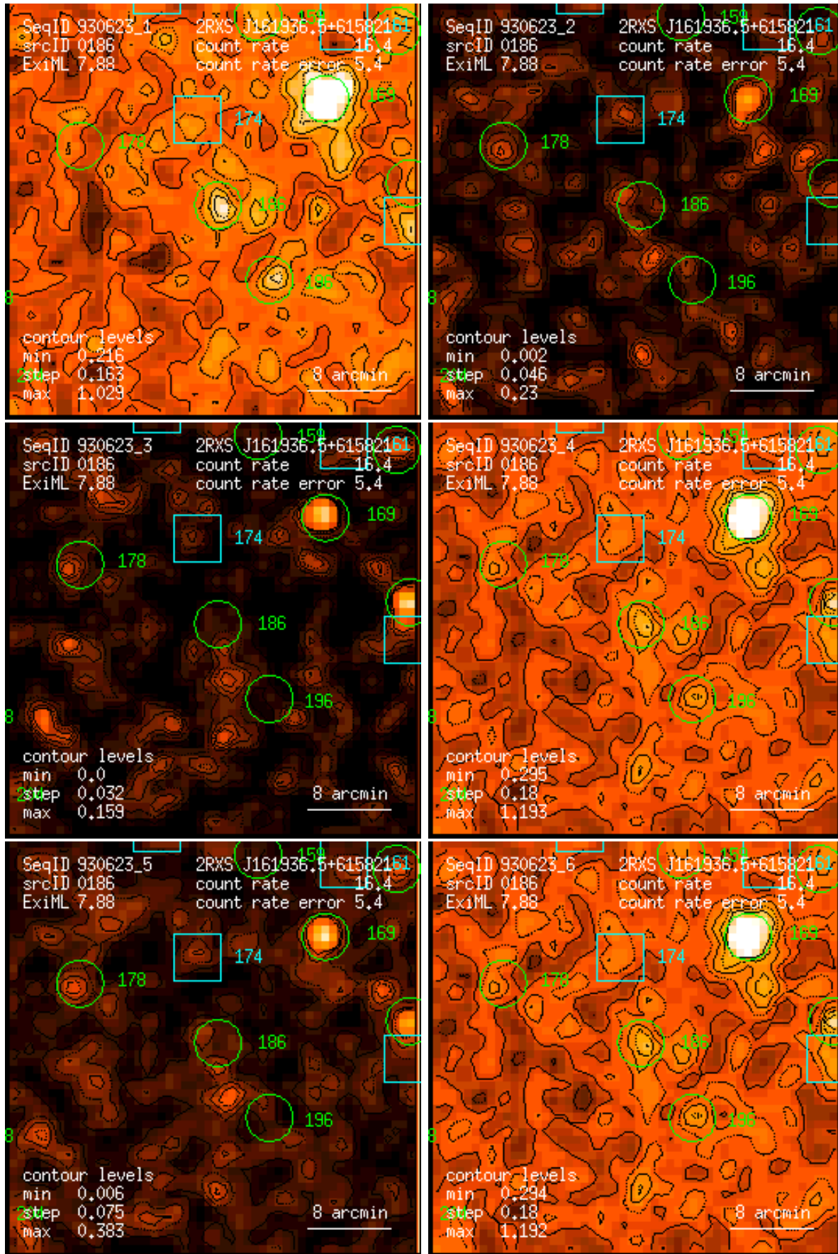
Figure 186: RASS 930623: detection 0186: band rate images, Gaussian filter: (1) PSPC channels 11 – 41, (2) 52 – 90, (3) 91 – 201, (4) 11 – 235, (5) 52 – 201, (6) 11 – 201. Broad band rates in counts/ks. Band rate contour levels in counts/ks/arcmin 2 .
