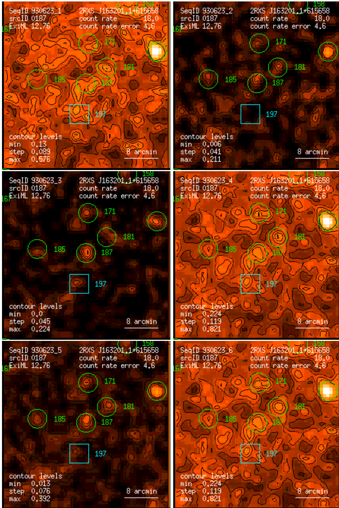
Figure 187: RASS 930623: detection 0187: band rate images, Gaussian filter: (1) PSPC channels 11 – 41, (2) 52 – 90, (3) 91 – 201, (4) 11 – 235, (5) 52 – 201, (6) 11 – 201. Broad band rates in counts/ks. Band rate contour levels in counts/ks/arcmin 2 .
