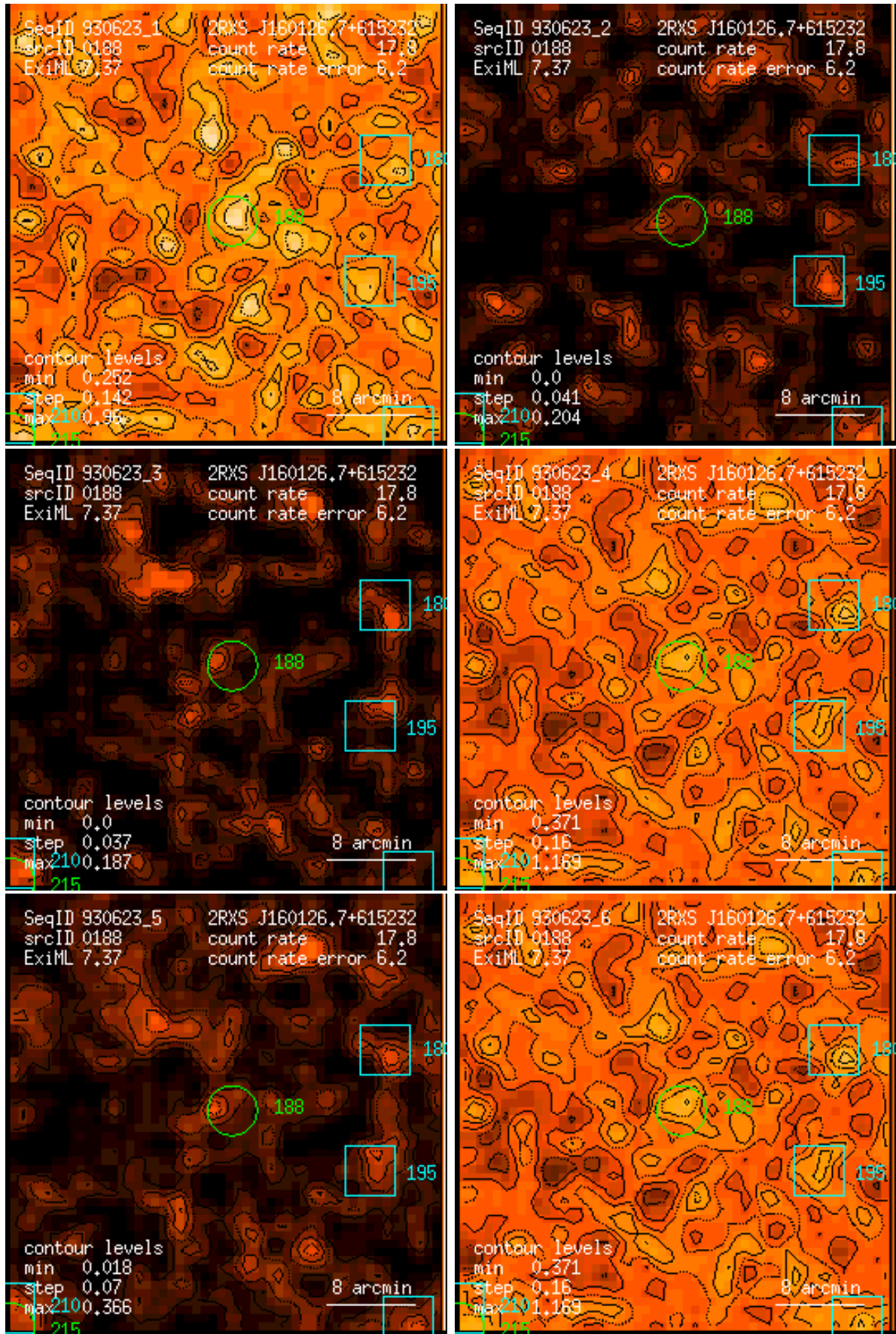
Figure 188: RASS 930623: detection 0188: band rate images, Gaussian filter: (1) PSPC channels 11 – 41, (2) 52 – 90, (3) 91 – 201, (4) 11 – 235, (5) 52 – 201, (6) 11 – 201. Broad band rates in counts/ks. Band rate contour levels in counts/ks/arcmin 2 .
