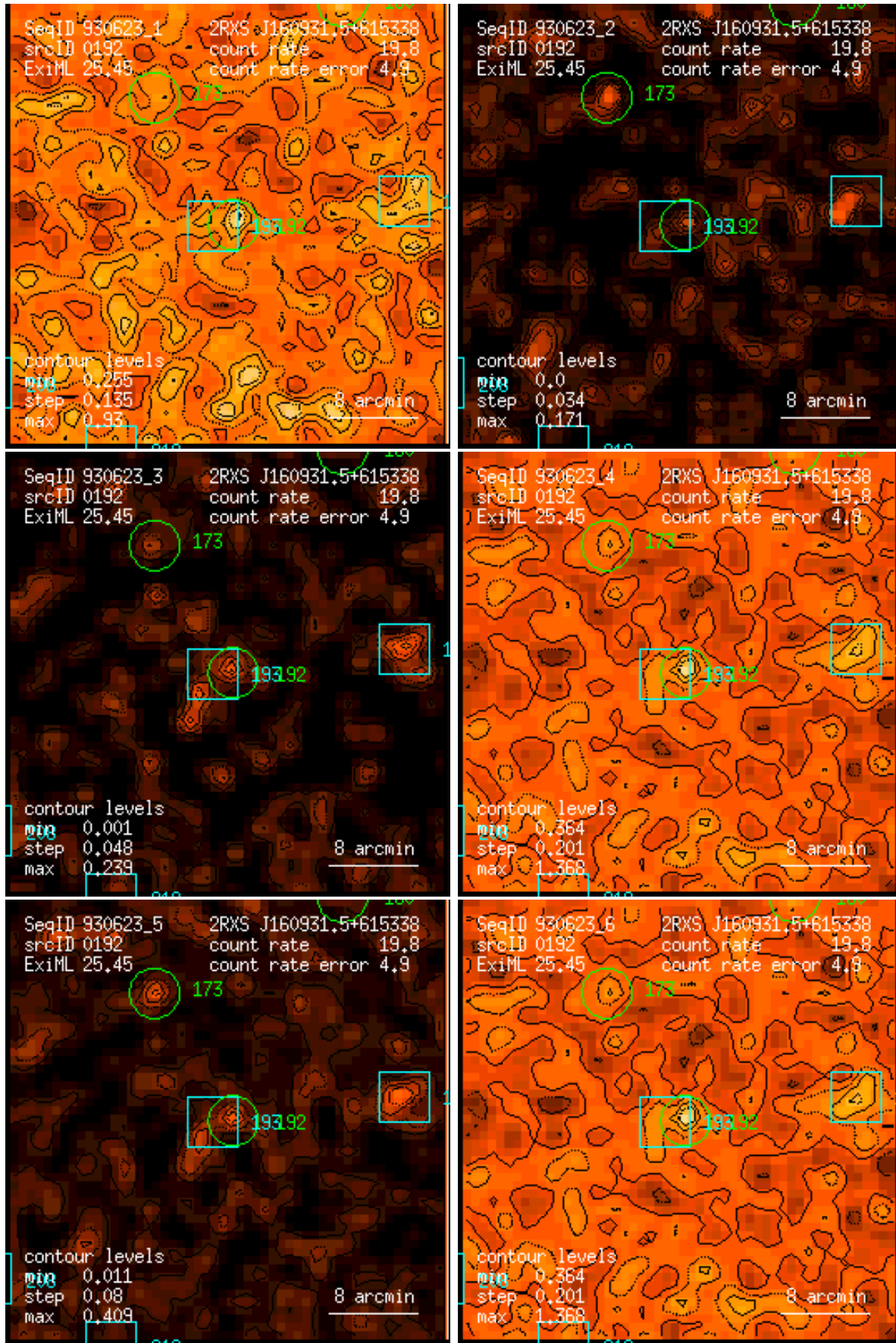
Figure 192: RASS 930623: detection 0192: band rate images, Gaussian filter: (1) PSPC channels 11 – 41, (2) 52 – 90, (3) 91 – 201, (4) 11 – 235, (5) 52 – 201, (6) 11 – 201. Broad band rates in counts/ks. Band rate contour levels in counts/ks/arcmin 2 .
