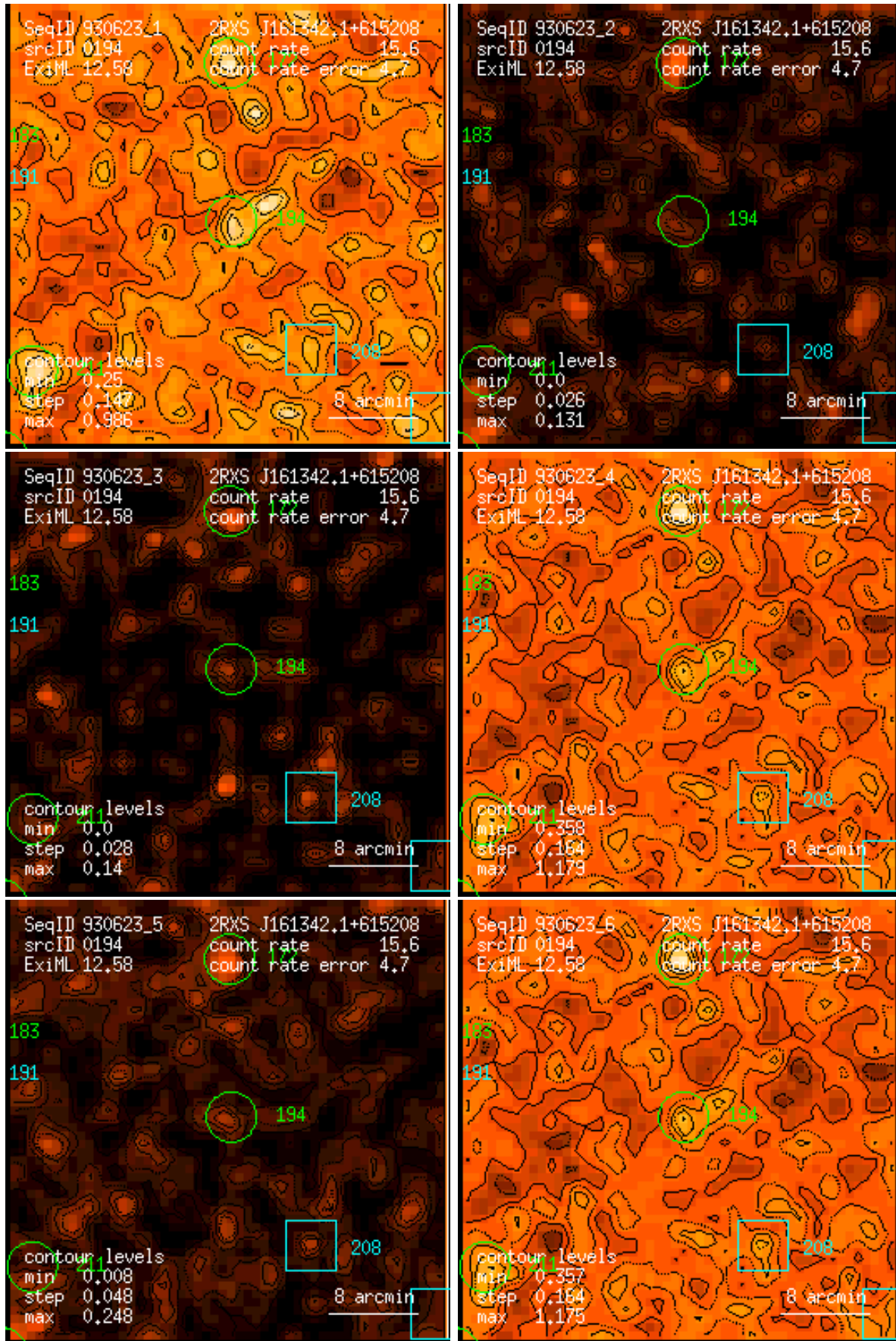
Figure 194: RASS 930623: detection 0194: band rate images, Gaussian filter: (1) PSPC channels 11 – 41, (2) 52 – 90, (3) 91 – 201, (4) 11 – 235, (5) 52 – 201, (6) 11 – 201. Broad band rates in counts/ks. Band rate contour levels in counts/ks/arcmin 2 .
